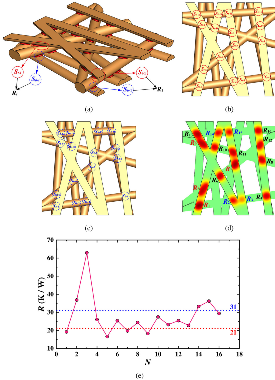
Fig. 13. Fibre solder joints: (a) schematic diagram of solder joints distribution; (b) distribution and numbering of top solder joints; (c) distribution and numbering of bottom solder joints; (d) thermal resistance distribution between top and bottom solder joints; (e) thermal resistance of solder joints.
