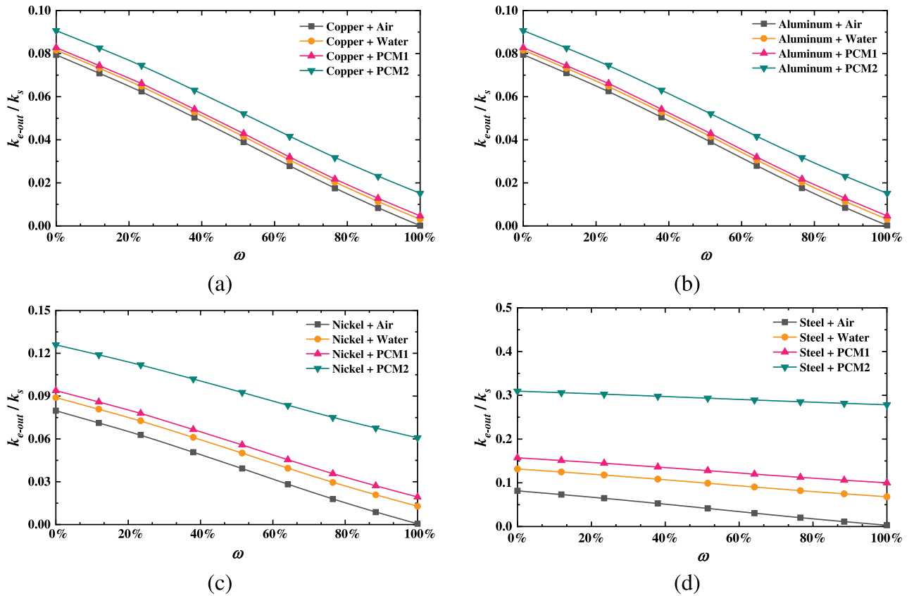
Fig. 17. Comparing the out-of-plane ETC of fibres with different filling fluids: (a) copper; (b) aluminum; (c) nickel; (d) steel.
