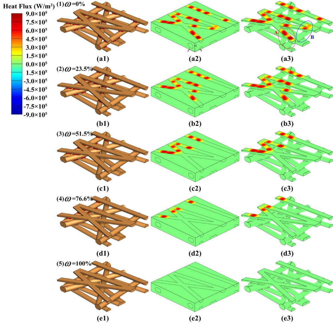
Fig. 11. Heat flux distribution for 2-D copper fibre with the different volume percentage of solder joint skips: (a) \omega = 0\% ; (b) \omega = 23.5\% ; (c) \omega = 51.5\% ; (d) \omega = 76.6\% ; (e) \omega = 100\% .
