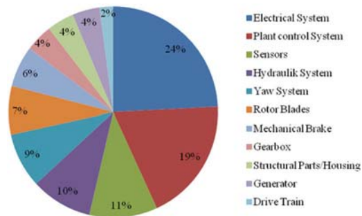
Figure 4. Failures percent of the main components.
