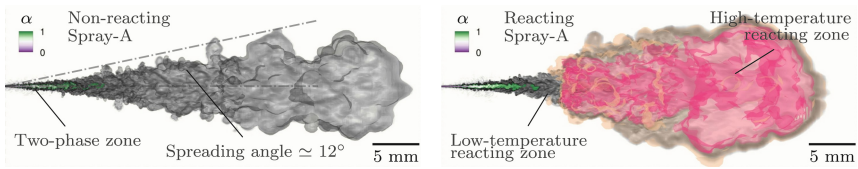
Fig. 4. LES-MT predictions of the inert (left) and reacting (right) ECN Spray A. Volume renderings at 800 \mu s after the start of injection.
