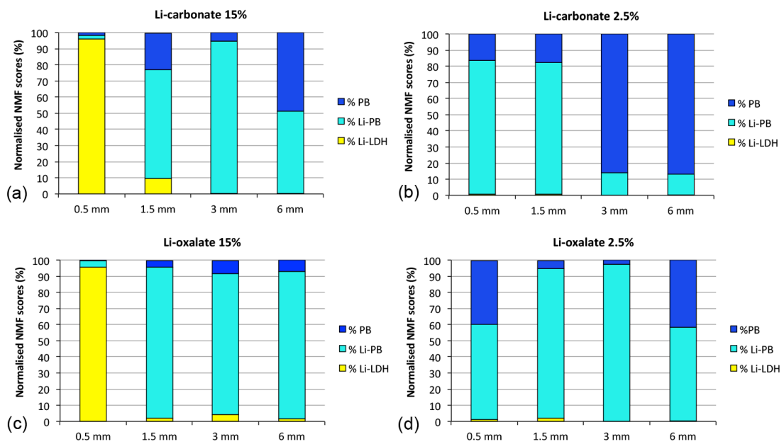
9 Fig. 11 Relative surface composition of the corrosion protective layer in the defect 10 areas (Li-LDH vs. Li-PB) obtained from the NMF image overlay data displayed in 11 Fig. 10: Li-carbonate loaded coating (a) 15% PVC; (b) 2.5% PVC and Li-oxalate 12 loaded coating (c) 15% PVC and (d) 2.5% PVC.
