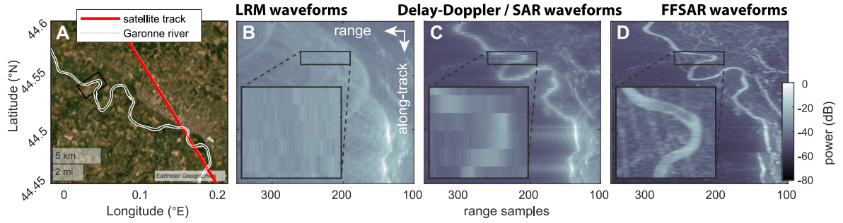
Fig. 1. The Garonne river as seen in different Sentinel-6 altimeter data products with varying along-track resolution due to differences in processing. Panel A shows the observation geometry. Panels B-D show the return signal in different altimeter data products: 20 Hz Low Resolution Mode (LRM) in which no SAR focusing has been performed (B), the 20 Hz SAR waveforms in which SAR focusing is performed over individual bursts of pulses (C) and the \sim 5917 Hz fully focused SAR waveforms, using a synthetic aperture of 2.2 s for SAR focusing (D). Single rows of the shown radargram are called waveforms.
