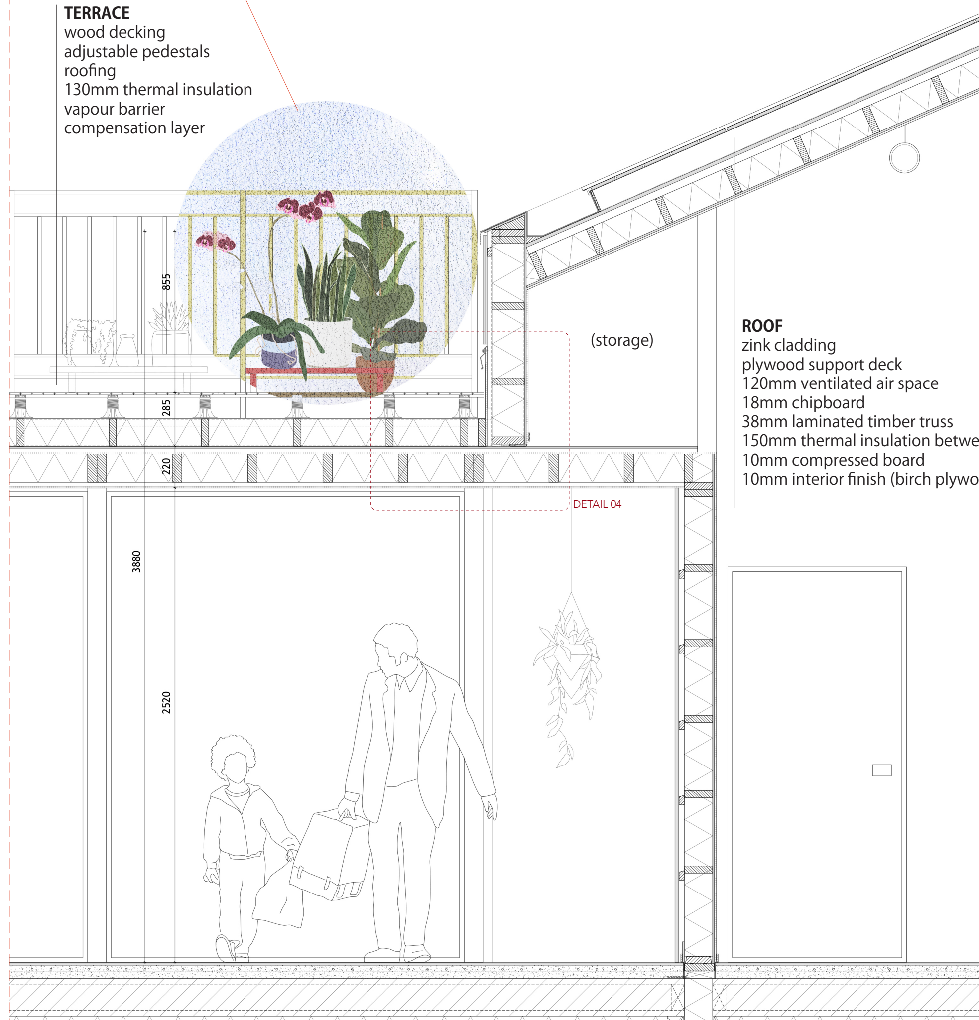
VERTICAL SECTION 2 scale 1:20
