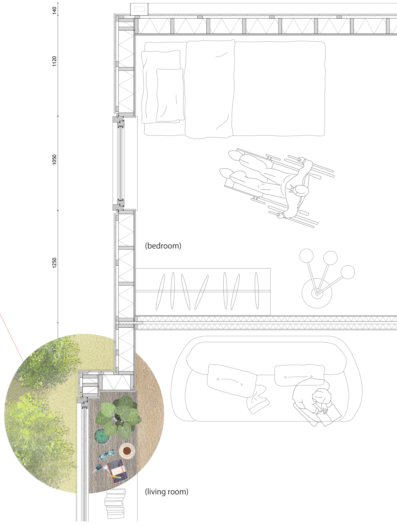
HORIZONTAL SECTION scale 1:20
