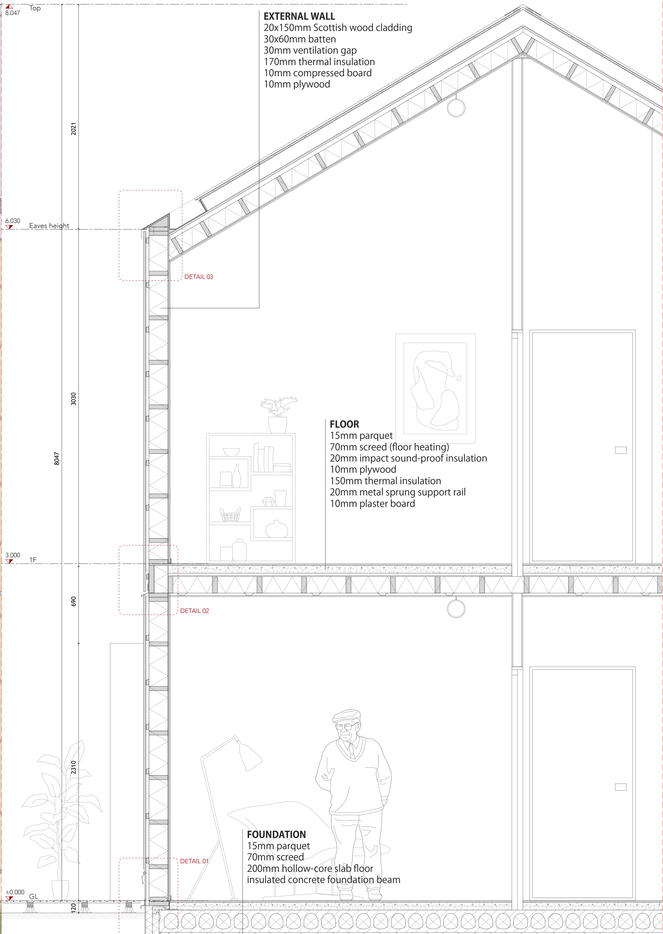
VERTICAL SECTION 1 scale 1:20
