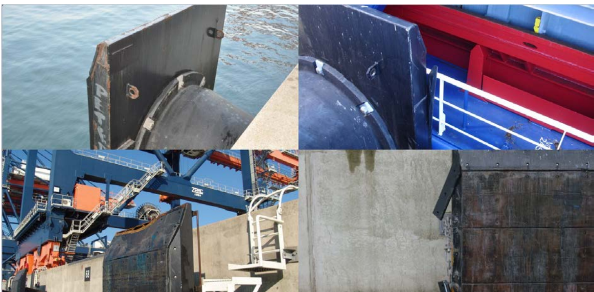
Figure 3: Damaged fender panels at Euromax Container Terminal Rotterdam (Photos PoR)
