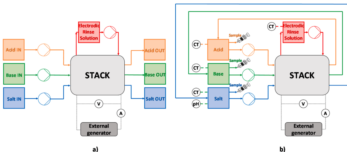
Fig. 5. Schemes of the experimental set-ups for a) once-through and b) closed-loop operations.
