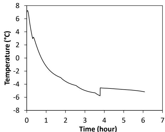
Fig. 6. Temperature profile of the feed solution.
