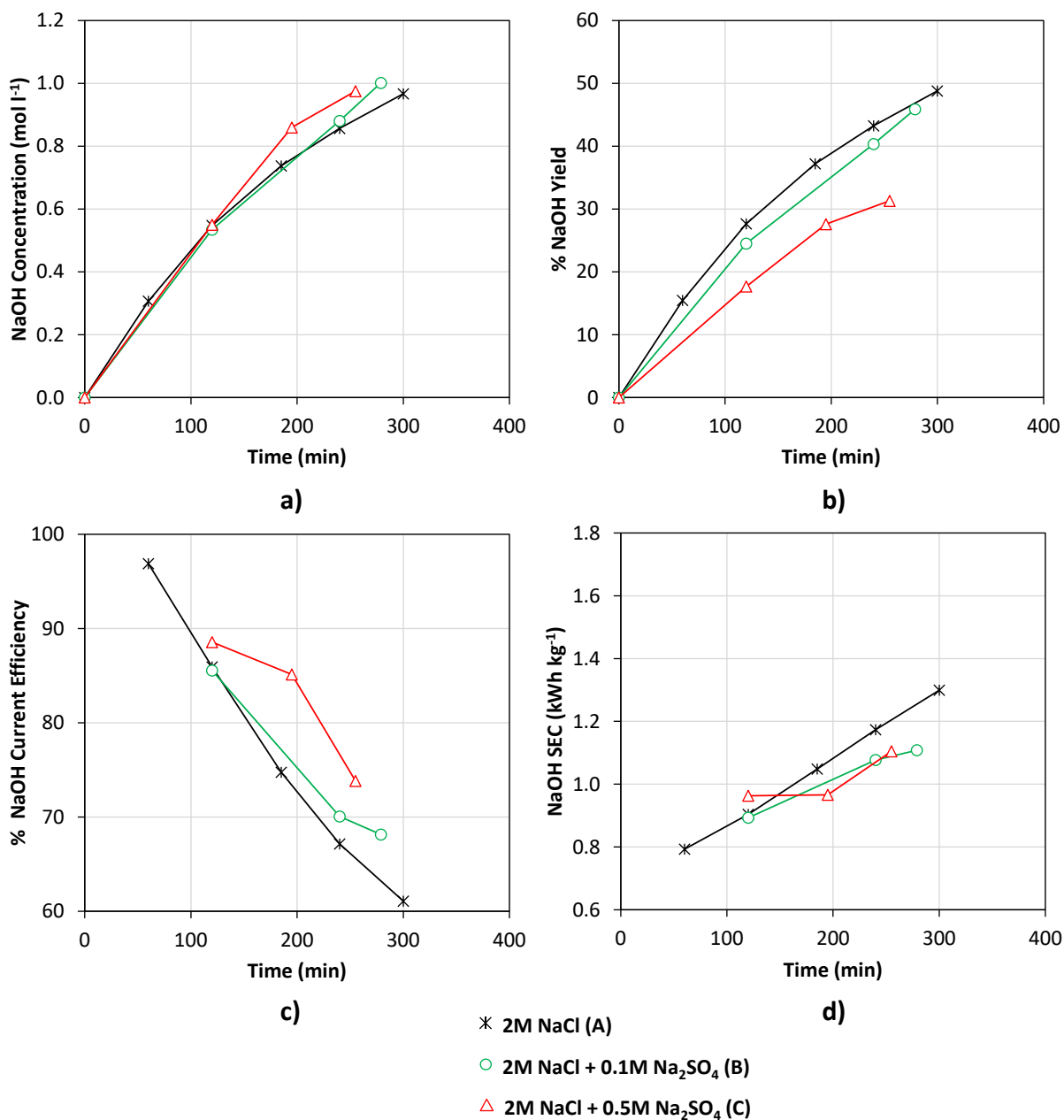
Fig. 12. Time dependency of a) Molar concentration of NaOH, b) % Yield of NaOH ( \tau ), c) % Current efficiency of NaOH ( \eta_c ) and d) Specific Energy Consumption of NaOH (SEC) as functions of time for a fixed current density of 100 \text{ A m}^{-2} in a closed-loop configuration. Inlet acid/base compartments: demineralized water.
