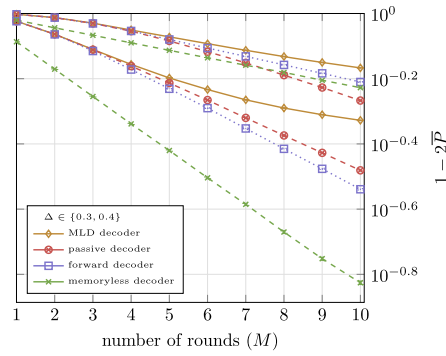
Figure 10. Logical error rate \bar{P} for decoding the circuit in figure 7 ( without the corrective displacement) for different decoders and squeezing parameters \Delta = 0.3 (top data) and 0.4 (bottom data) with the number of stabilizer measurement rounds M = 1, \dots, 10 . For \Delta = 0.3 the mean performance of the forward decoder outperforms passive decoding, while the opposite is true for \Delta = 0.4 . We have observed that the single sample logical error rates strongly fluctuate at O(10^{-2}) - O(10^{-1}) around the averages, suggesting rather chaotic behavior. The data are obtained by sampling over N = 5 \times 10^4 trajectories of measurement outcomes. Error bars denote the standard deviations of the averaged logical error rates. The memoryless decoder applies a different corrective displacement after each QEC round described in appendix B.
