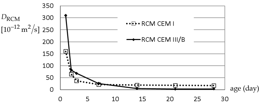
Figure 1: Evolution of instantaneous diffusion coefficient (RCM) with time
