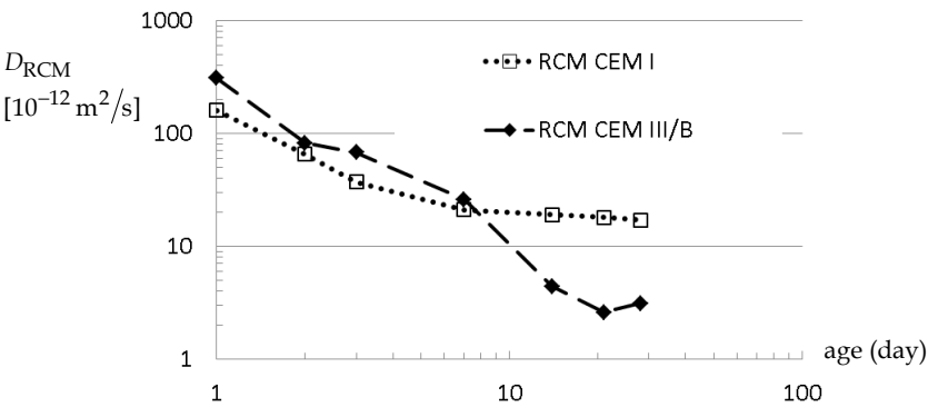
Figure 2: Logarithmic evolution of instantaneous diffusion coefficient (RCM) with logarithm of time
