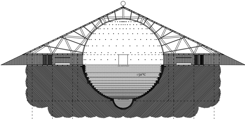
-section-
