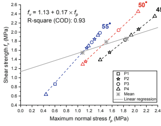
Fig. 6. Failure envelope from splitting tests on cores using: (a) the average result for each inclination; (b) all data.
