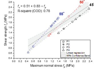
Fig. 6. Failure envelope from splitting tests on cores using: (a) the average result for each inclination; (b) all data.
