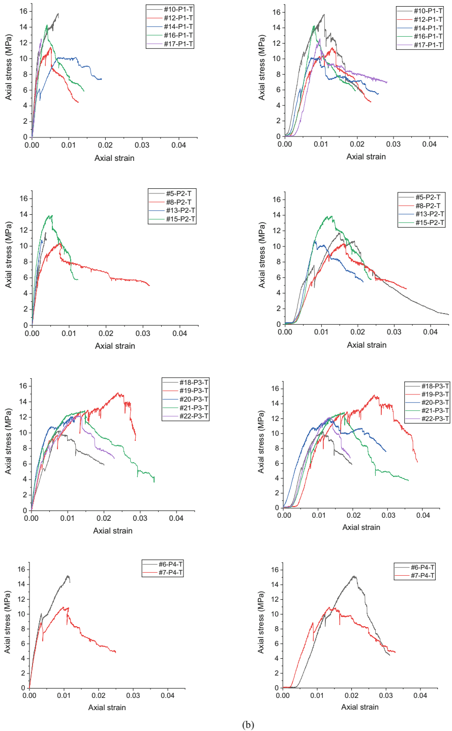
Fig. 10. Compression behaviour of T-shaped cores from Piece 1 to 4: (a) normal strain obtained by LVDT's reading; (b) normal strain obtained by jack's reading.
