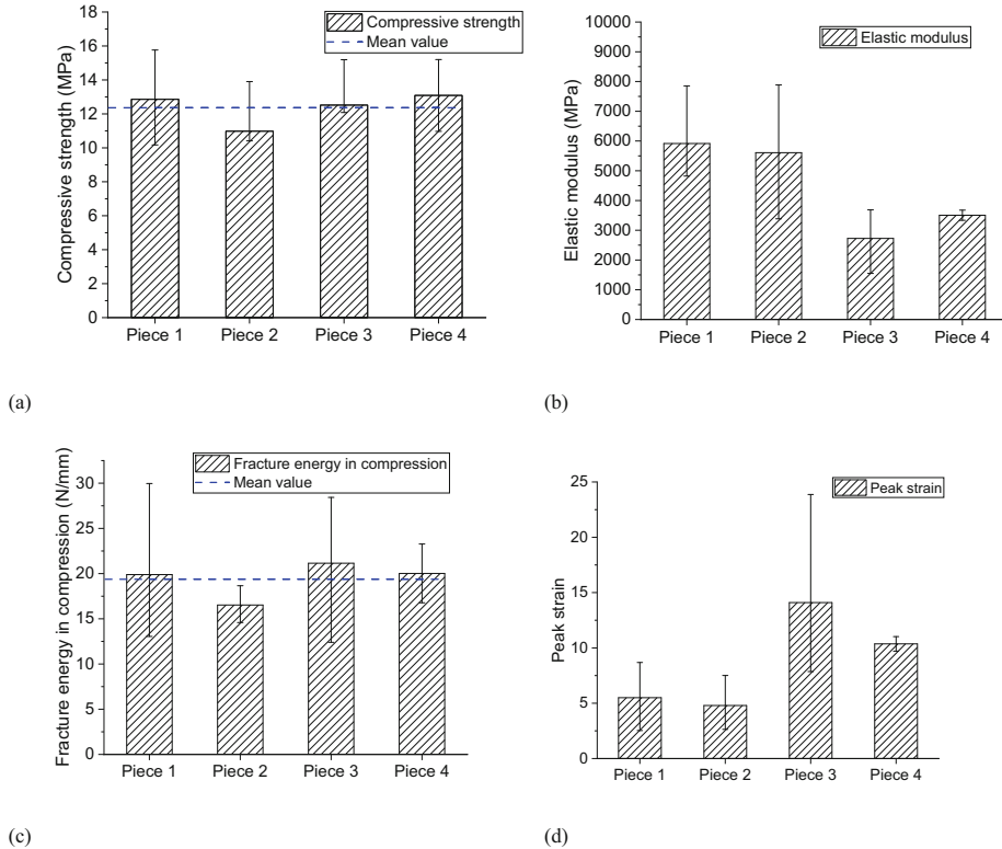
Fig. 11. Mean value of compressive properties for each Piece (Piece 1 external, Piece 4 internal): (a) Compressive strength (b) Elastic modulus (c) Fracture energy in compression (d) Peak strain.
