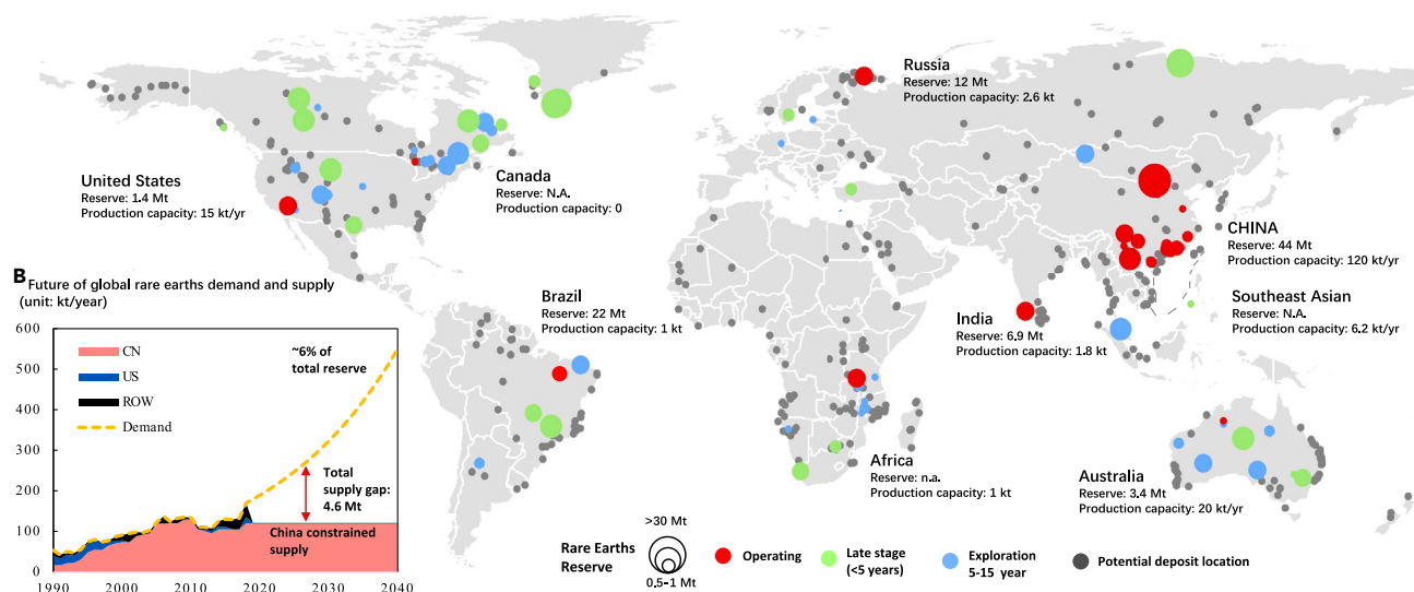
Figure 5. Global distribution of advanced REs projects, and future demand and supply
