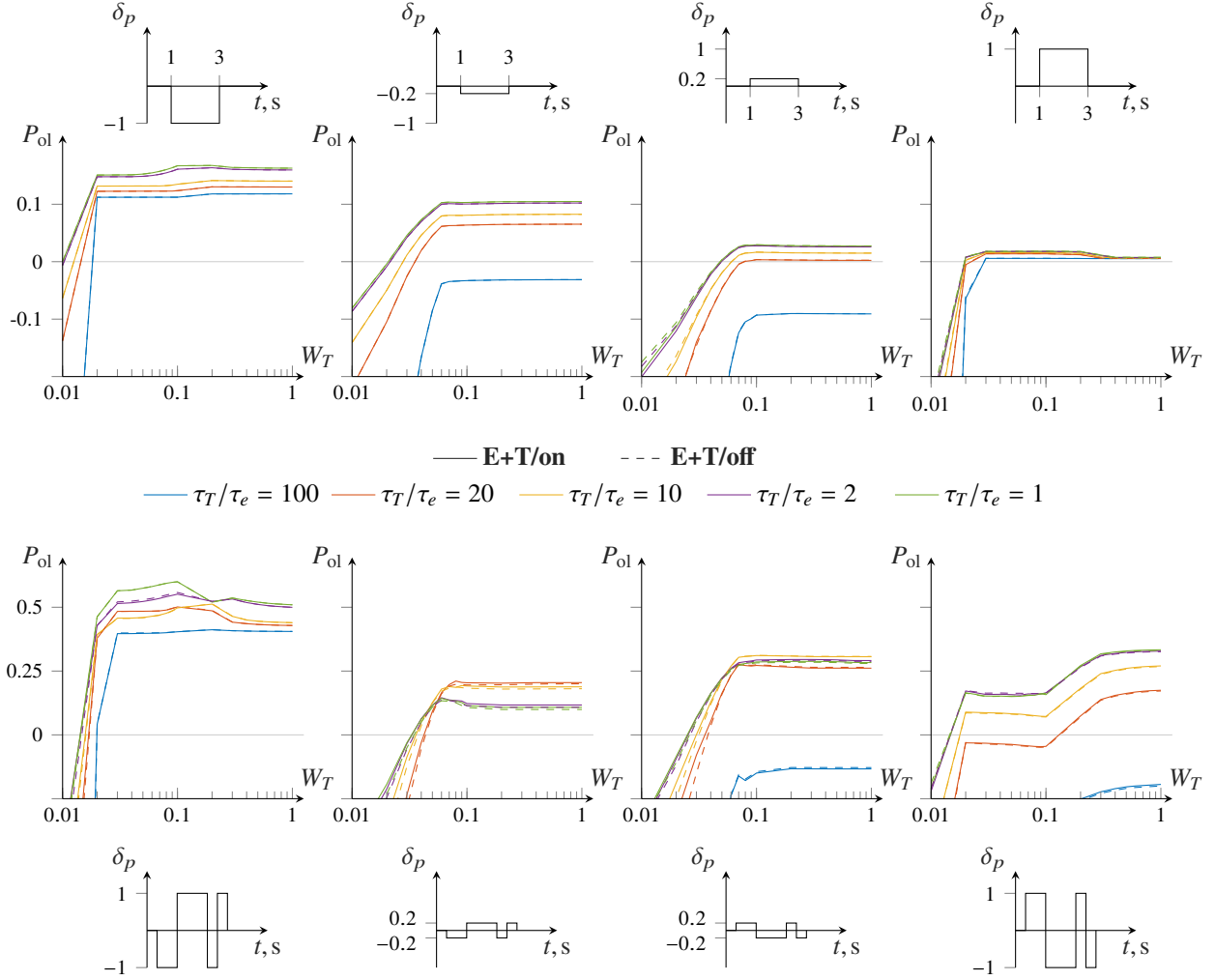
Fig. 10 Open-loop performance benefit as a function of thrust allocation weight W_T and non-linear allocation filter f_W . Elevator actuator speed \tau_e = 0.05 s. Trim conditions as in Fig. 5. (Top row) 2 s impulse maneuver. (Bottom row) 2-3-1-1 maneuver.
