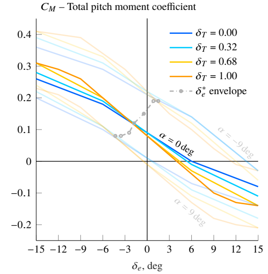
Fig. 4 Total pitch moment coefficient C_M for the DUUC. CFD simulations at V = 80 m/s.
