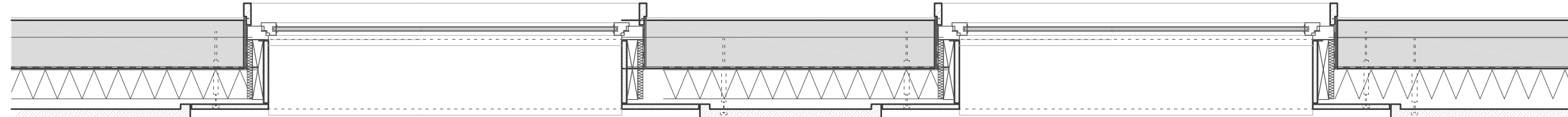
Horizontal section B 1:20
