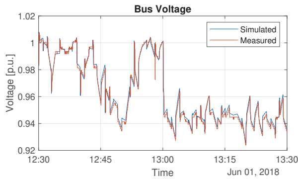
Fig. 4: Simulated (Newton-Raphson) and measured phase voltage (output of power amplifier). The base value is 230 V.
