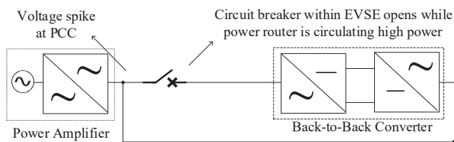
Fig. 7: Breaking the loop at high circulating power.
