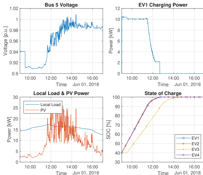
Fig. 10: Experimental results for uncontrolled charging with demonstrator EV attached at node-5 in the test-grid. EV 1, 2 and 4 have a capacity of 50 kWh and arrive at 9:00. For EV 3 this is 100 kWh and 9:30.
