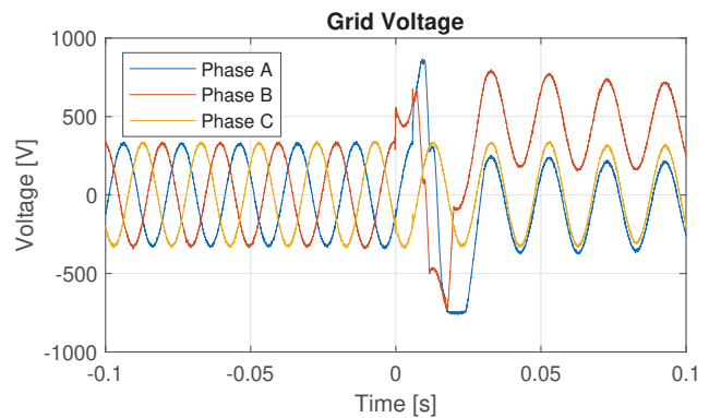
Fig. 8: Phase voltages when current is interrupted at t = 0 .
