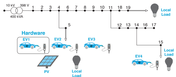
Fig. 3: Single-line diagram of a Dutch grid used for grid simulation
