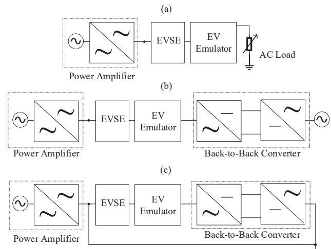
Fig. 5: Available power routing options (a) AC Load (b) grid-connected (c) circulating power
