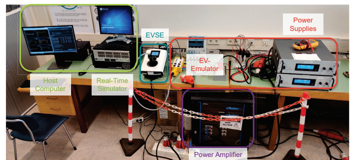
Fig. 9: Picture of experimental setup
