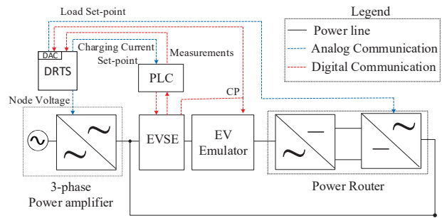
Fig. 2: Block diagram of the experimental implementation of Fig. 1. Solid lines represent power flows and dotted lines information flows.
