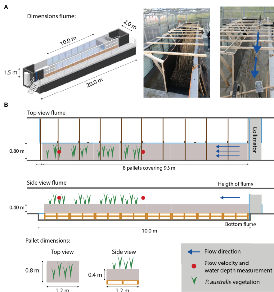
FIGURE 2 | Overview of the flume dimensions and experimental setup (A). Schematic top view and side view of the experimental setup in the flume (B). The flow is generated by a pump that forces water through a collimator into the 0.80 m wide test section. Uniform flow was created by removal of the aboveground vegetation in the first meters of the test section.
