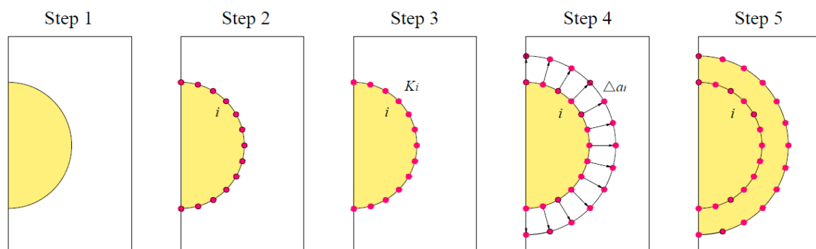
Figure 9. Five steps of the adaptive re-meshing technique [19].
