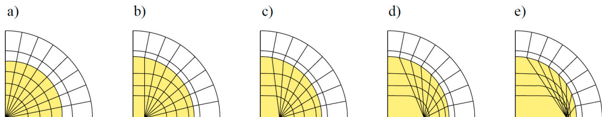
Figure 8. Five degrees (a-e) of mesh non-orthogonality, from an orthogonal mesh to a distorted mesh [48].
