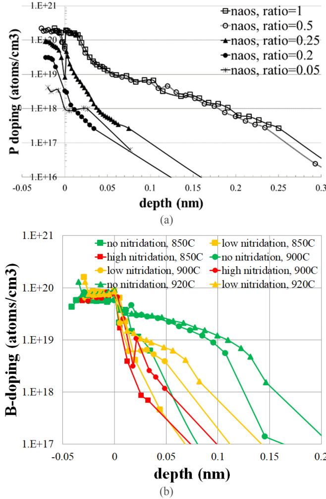
FIGURE 2. ECV profiles for (a) P doping for different ratios ( n/(n+i) ) using NAOS as interfacial layer, and (b) B-doping (40nm layers) on wafers with NAOS annealed at 850, 900 and 920°C which received high, low or no amount of nitridation.
