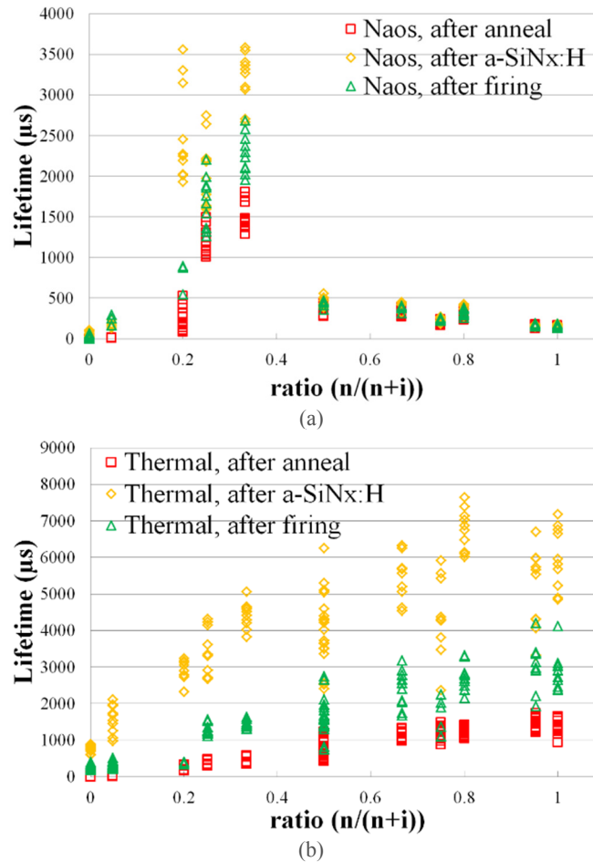
FIGURE 1. Minority carrier lifetime as function of the ratio ( n/(n+i) ) with NAOS (a) and thermal oxide (b) as interfacial layer, as measured after anneal, after a-SiNx:H deposition and after firing.
