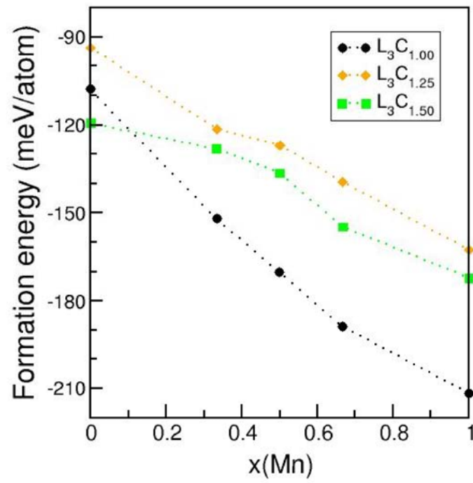
Figure 6: Formation energy of the O and M-carbide phases as a function of the Mn content x , whereby the chemical composition is given by the formula [\text{Mn}_x\text{Cr}_{(1-x)}]_3\text{C}_y . The three curves are for different C concentrations ( y=1.0, 1.25, 1.5 ).
