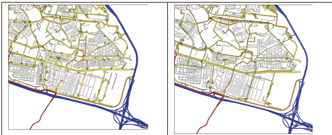
Figure 2 Thinning of the road network before (left) and after (right) generalisation (displayed with same symbol size and at same scale)
