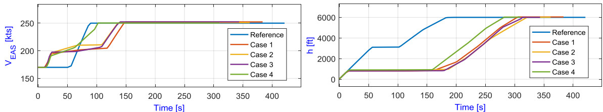
Fig. 5. Vertical profiles of cases 1-4 and the reference case.
