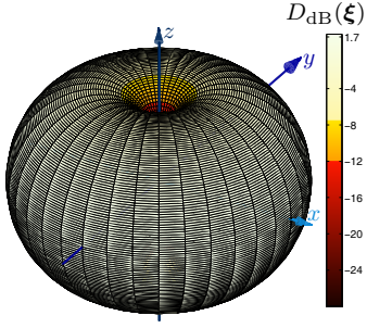
Fig. 3. D_{dB}(\xi) pattern for a rhombic antenna rotated by \varphi_R = 90^\circ ; excitation: a train of 5 dPE pulses with a R_r pulse repetition rate.
