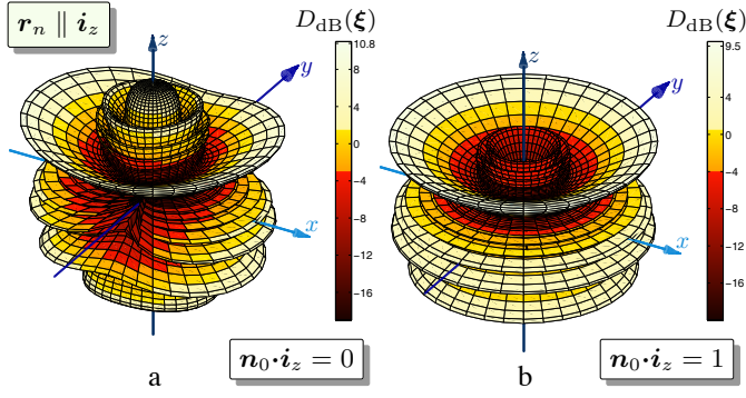
Fig. 7. D_{dB}(\xi) pattern for a uniform, linear array consisting of 8 rhombic antennas; excitation: a train of 5 d t PE pulses with a R_r pulse repetition rate; inter-element spacing: c_0 R_r/2 ; beam steered at \xi_{st}, i_z = 30^\circ .
