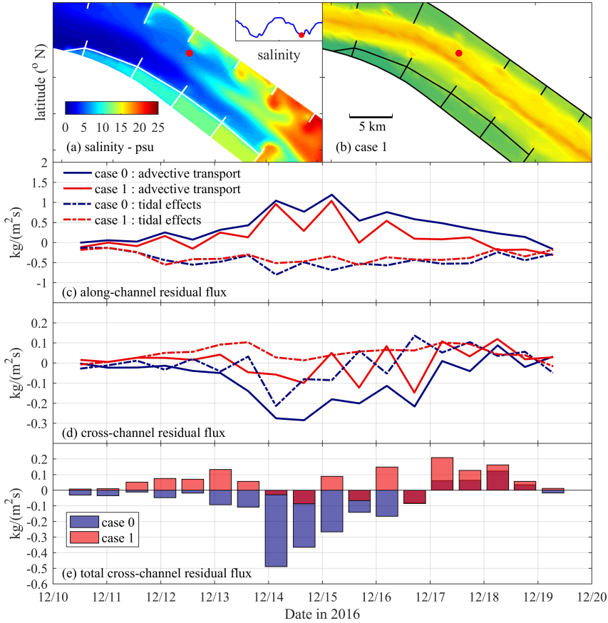
Figure 3.13: Numerical cases setting and single-point residual sediment flux, case 0: standard case with near-bed salinity distribution during low water slack (a); case 1: the groyne nearest to the observational site is removed, marked with white rectangle (b); decompositions of residual flux at the observational site in along-channel (c) and cross-channel (d) direction; and difference of cross-channel residual flux between case 0 and case 1 (e). The positive value in (c) indicates direction of about 120 degrees from the north, the positive value in (d) indicates direction of about 30 degrees from the north.
