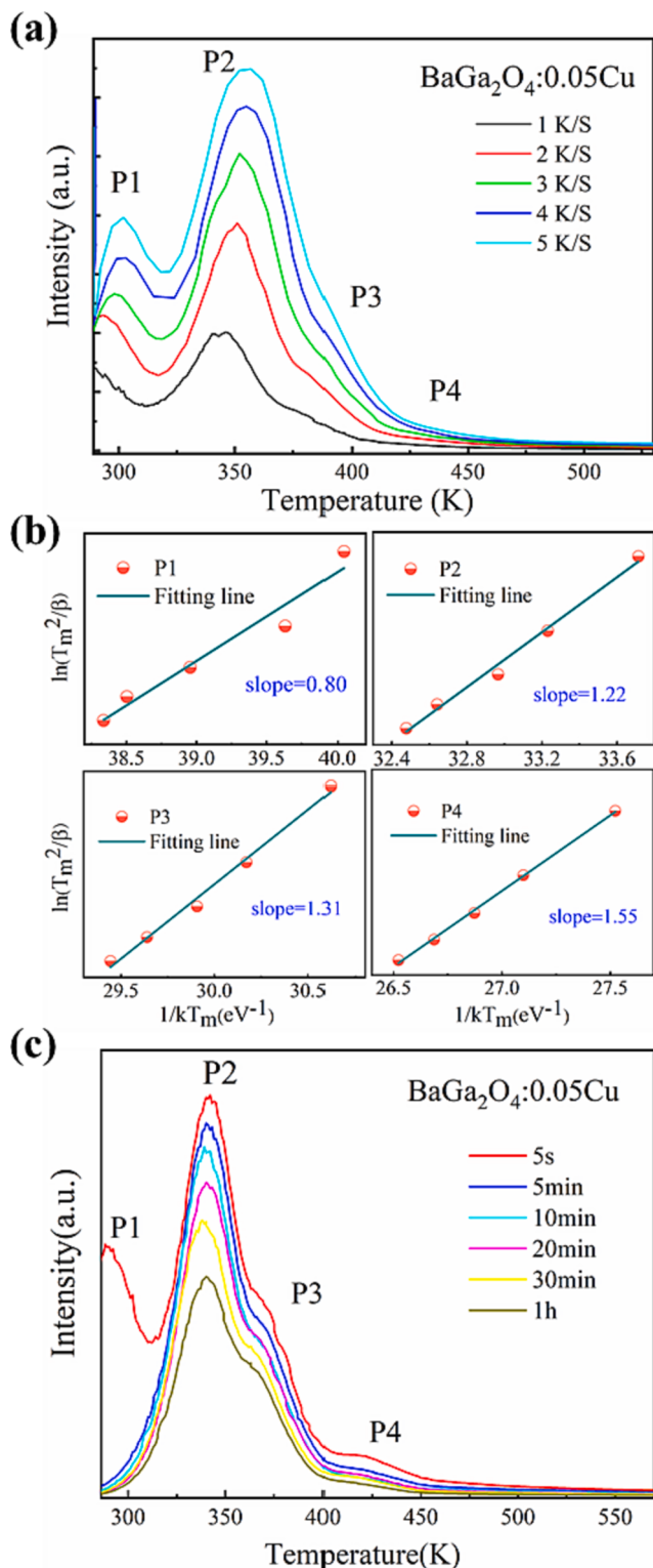
Fig. 7. (a) TL spectra of \text{Ba}_{0.95}\text{Ga}_2\text{O}_4:0.05\text{Cu} collected after irradiation with both 254 and 365 nm for 5 min. (b) Relationships between \ln(T_m^2/\beta) and 1/kT_m of the four peaks in (a). (c) TL curves of \text{Ba}_{0.95}\text{Ga}_2\text{O}_4:0.05\text{Cu} recorded at different decay times after removing the UV lamps.
