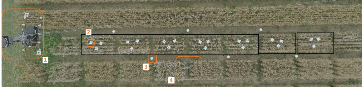
Figure 3. Overview of experiment setup and data collection. Orange rectangles: (1) field phenotyping platform with a camera rig, (2) photogrammetric target (coded marker), (3) reference sphere, (4) TLS. Black rectangles: 7 wheat plots covered within a measurement campaign, from left to right - 5 training, 1 validation, 1 test / hold-out plot.
