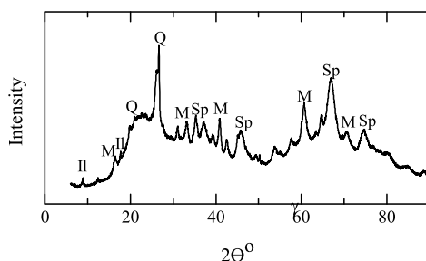
Figure 6.1: XRD patterns of the calcined kaolin samples identifying the main mineral phases. Il = illite, Q = quartz, Sp = Al-spinel, M = mullite.
