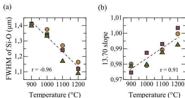
Figure 5.6: Spectral parameters that describe the redefinition of the Si–O and Al–O features in the high-temperature domain. (a) FWHM of the Si–O feature around 9.50 \mu\text{m} ; (b) 13.70 slope parameter that indicates the formation of the Al–O absorption band. ( \square = K1, \bullet = K2, \blacktriangle = K3).
