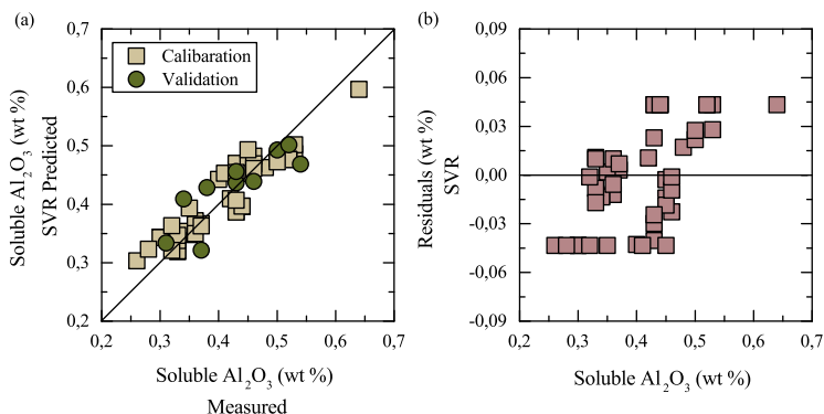
Figure 6.9: (a) Measured vs Predicted plot of the SVR model for the 5.7 to 6.5 \mu\text{m} range after CR processing. C = 3.1 , \epsilon = 0.46 , SV = 19 in the calibration and validation samples. (b) Residuals plot of the SVR calibration.
