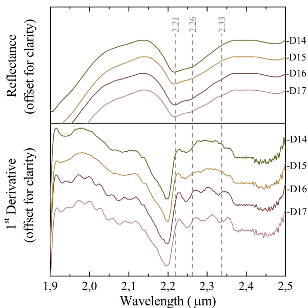
Figure 10.6: Bidirectional reflectance spectra of diatomite ore samples with variable content of \text{CaCO}_3 after continuum removal ( top ) and 1 st derivative ( bottom ): D14 = 6.29 wt%, D15 = 10.9 wt%, D16 = 16.4 wt%, D17 = 24.4 wt%. The dashed lines indicate position of the spectral features opal (2.21 and 2.26 \mu\text{m} ) and calcite and aragonite (2.26 and 2.33 \mu\text{m} )
