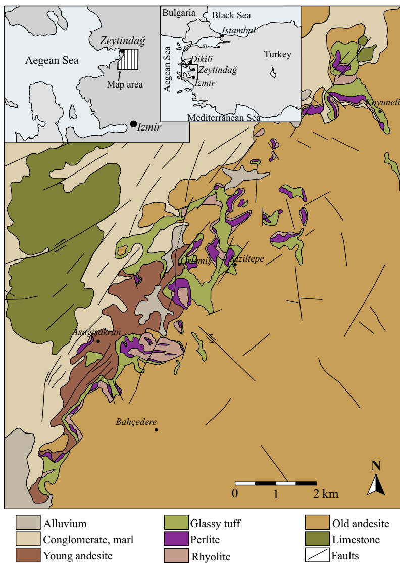
Figure 9.1: Distribution of the Zeytindağ perlite deposits in the Dikili – İzmir area (Reproduced after Özgenc (2012), with permission)
