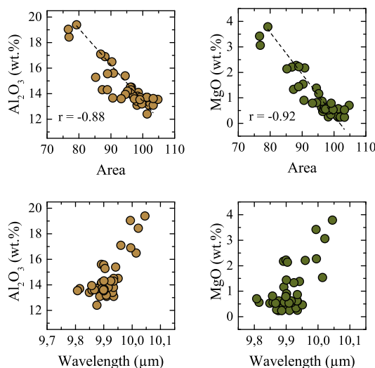
Figure 9.4: Correlation between spectral parameters and \text{Al}_2\text{O}_3 and MgO indicating that small area and long wavelength values indicate the presence of montmorillonite (Error bars smaller than plot symbol)
