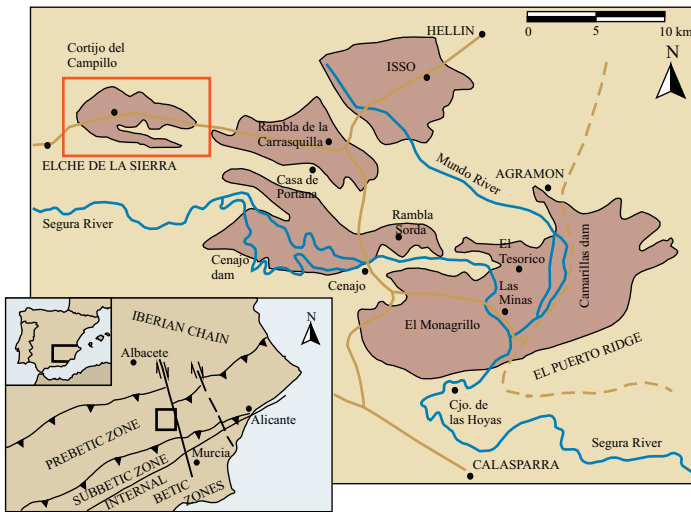
Figure 10.2: Neogene basins on the external side of the Betic Ranges, and location of the Elche de la Sierra basin (red rectangle in the upper-left corner) (Modified from Ortí et al. (2014), with premission)
