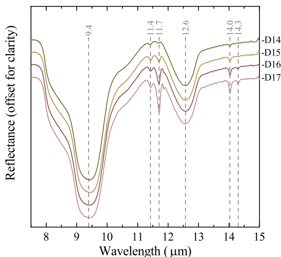
Figure 10.5: Attenuated total reflection (ATR) infrared (IR) spectra of diatomite ore samples with variable content of \text{CaCO}_3 : D14 = 6.29 wt %, D15 = 10.9 wt %, D16 = 16.4 wt %, D17 = 24.4 wt %. The dashed lines indicate position of the spectral features opal (9.4 and 12.6 \mu\text{m} ), calcite (11.4 and 14.0 \mu\text{m} ) and aragonite (11.7, 14.0 and 14.3 \mu\text{m} )
