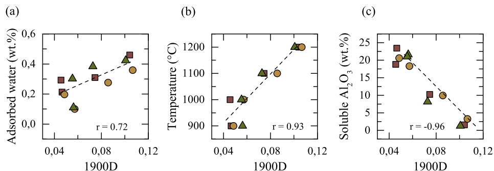
Figure 5.10: Variation in the depth of the 1.9\mu\text{m} absorption band (1900D parameter) compared with the changes in (a) adsorbed water, (b) temperature and (c) soluble \text{Al}_2\text{O}_3 ( \square = K1, \circ = K2, \triangle = K3) (Error bars smaller than plot symbol).
