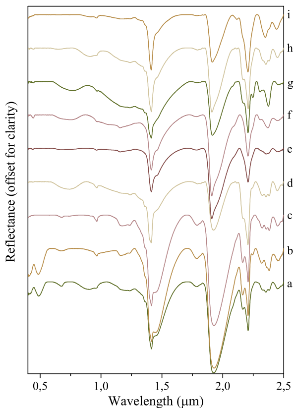
Figure 4.5: Minerals present in the kaolinised granite samples from the St Austel Granite that have characteristic spectral features in the SWIR range. The samples were collected at (a) Littlejons pit, (b–d) Melbur pit and (e–i) Virginia pit. (a) kaolinite, muscovite, illite, goethite, hematite; (b) kaolinite, goethite, biotite; (c) kaolinite, biotite; (d) kaolinite, biotite, muscovite; (e) montmorillonite, muscovite; (f) montmorillonite, muscovite, biotite; (g) tourmaline, biotite, montmorillonite, kaolinite; (h) kaolinite, montmorillonite, muscovite, hematite; (i) muscovite, goethite
