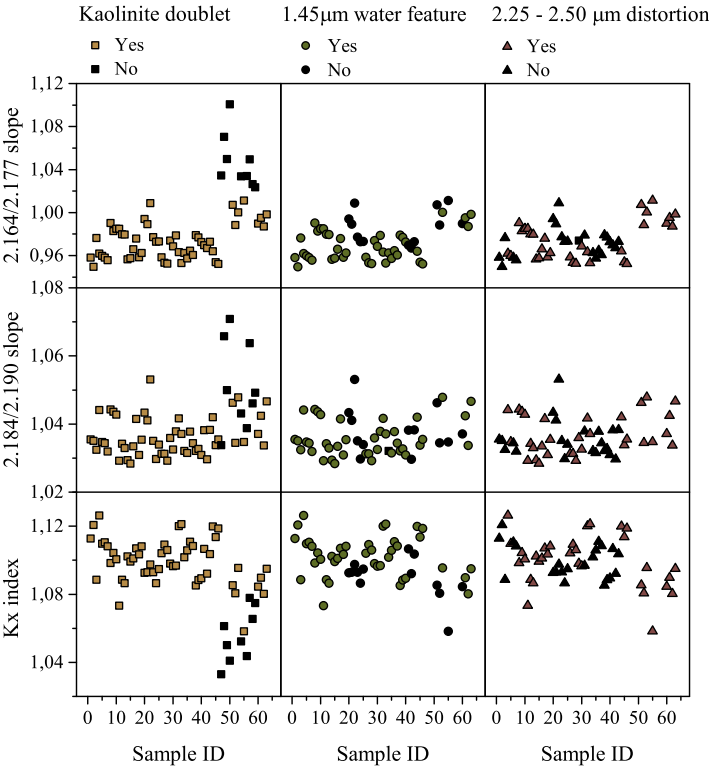
Figure 4.9: Slope parameters and Kx index values calculated from the point spectra, compared to the presence of the kaolinite 2.2 µm doublet, the 1.45 µm water absorption and the kaolinite spectral distortions in the 2.25 to 2.50 µm range. .
