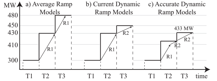
Fig. 1: Different ramp-rate models
