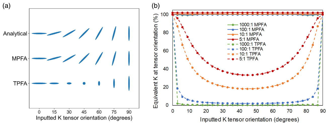
Figure 4. (a) Effective conductivity ellipsoids for two-point flux approximation (TPFA) and multipoint flux approximation (MPFA, implemented using the XT3D option) compared to the analytical for K_{\text{max}}:K_{\text{min}} of 10:1. (b) Effective conductivity as a percentage of the analytical value for various tensor angles, anisotropy ratios and numerical scheme (TPFA vs. MPFA).
