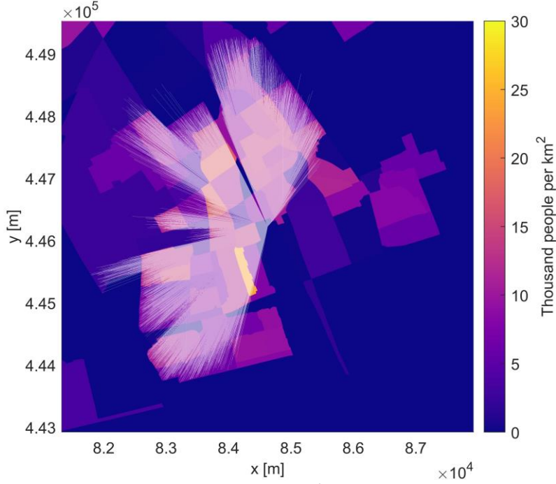
Figure 6: UA Flight Paths with \hat{R}_{Cground}^i / T_i^{nom} > 10^{-6}
