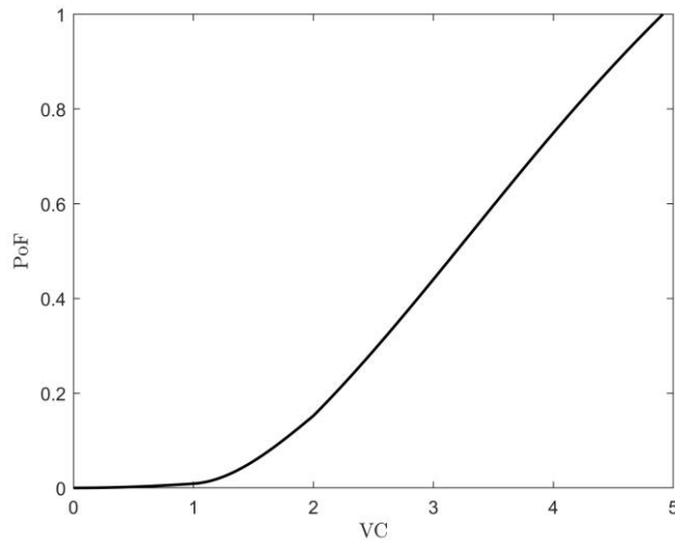
Figure C6. Conversion of VC injury level to PoF
