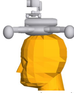
Figure 3. Scenario A impact at center of gravity of human head, i.e. \Delta = (0,0)
