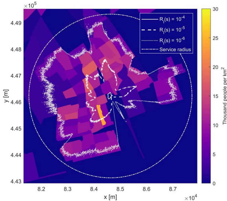
Figure 8: Individual Risk Contours of \hat{R}_I^{UAS}(j) = 10^{-6} , 10^{-5} and 10^{-4} projected on population map in Figure 1.
