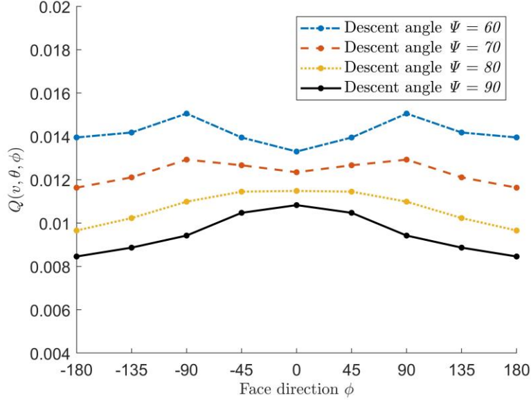
Figure 9. Q(v, \theta, \phi) as a function of face direction and descent angle at \theta_{pitch} = 150^\circ , |v| = 18m/s
