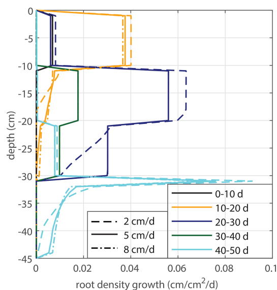
Figure 6. Sensitivity of root growth profiles to different values of the vertical root growth rate u_1 . The different colors refer to the consecutive time periods of Fig. 5; i.e., the graphs represent 10 d averages of the daily root density growth rates.
