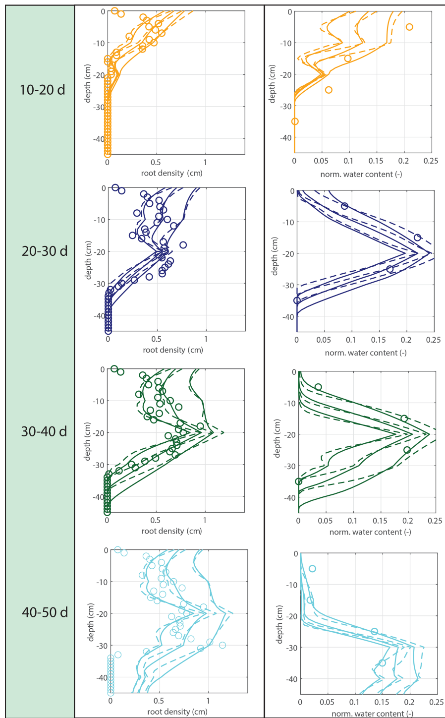
Figure 14. Comparison of results for loamy sand (solid lines) and sandy loam (dashed lines) for three different values for u_2 ( 0.6 \times 10^{-2} , 1.2 \times 10^{-2} , and 2.4 \times 10^{-2} \text{ mL cm}^{-1} \text{ h}^{-1} ).
