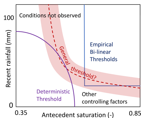
Figure 3. Different formats of hydrometeorological thresholds for landslide initiation developed based on empirical interpretation (blue), shown with bilinear thresholds optimized using several years of monitoring data and landslide inventories (Mirus et al., 2018), versus theoretical understanding (purple) based on a deterministic method using infiltration modeling and millions of synthetic storm events (Thomas et al., 2018). The deterministic threshold shows unconditionally unstable conditions for excessive rainfall or high saturation levels. In contrast, empirical thresholds indicate that excessive rainfall on dry soils will not trigger failures, whereas even at the highest observed saturations moderate rainfall is still needed to trigger failures. Heuristically, a general threshold that accommodates both theoretical understanding and empirical observations seems more reasonable.
