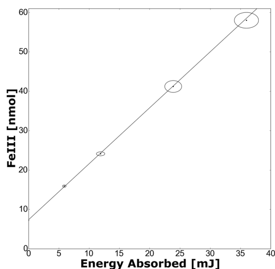
Figure 2. Measured amount of Fe 3+ as a function of radiation energy absorbed by the sample. The slope of the line of best fit through the data is the G-value ( 1.42 \pm 0.08 \mu\text{mol/J} ). Error bars (indicated by ellipses) are \pm two standard errors and indicate statistical errors alone. These measurements were taken with a dose rate of 150 \pm 20 \text{ Gy/s} .
