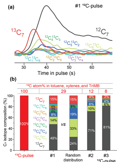
Figure 3. Contributions of \text{C}_7 aromatics (formula ^{12}\text{C}_n^{13}\text{C}_{7-n} , n = 0 – 7 ) from MS responses at m/z = 91 – 98 corrected for fragmentation upon the first ^{12}\text{C} -MeOH pulse after repetitive pulsing ^{13}\text{C} -MeOH (top) and corresponding \text{C}_7 isotope composition (bottom) with the ^{13}\text{C} content (at %) in the last ^{13}\text{C} -MeOH pulse response and the following three ^{12}\text{C} -MeOH pulse responses, pulse interval = 3.75 min. The ^{13}\text{C} content in the displacement peak, m/z = 98 is not taken into account to estimate the random distribution of ^{13}\text{C} in m/z = 91 – 98 aromatic fragments.
