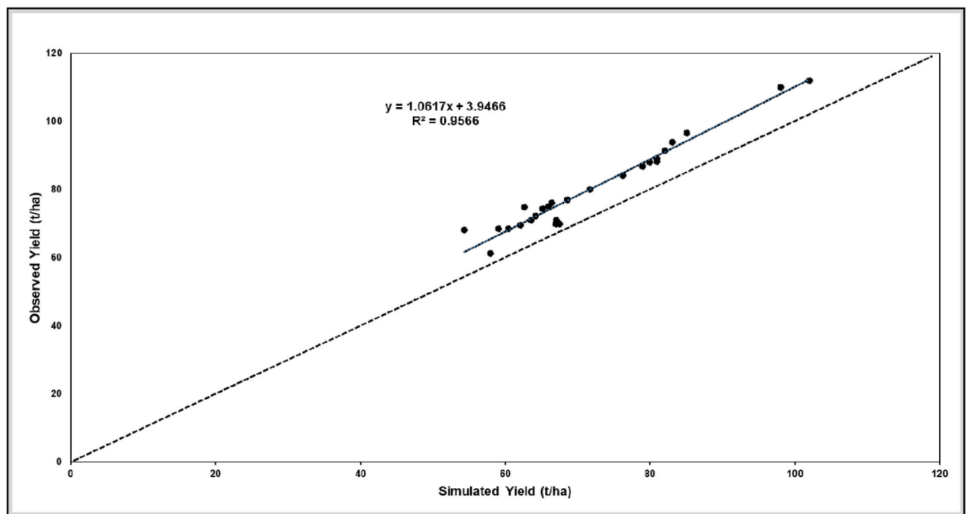
Fig. 5. AquaCrop verification results based on average (i.e. combined) observed ( Y_a ) and simulated ( Y_p ) sugarcane yield data for the mill areas in South Africa.
