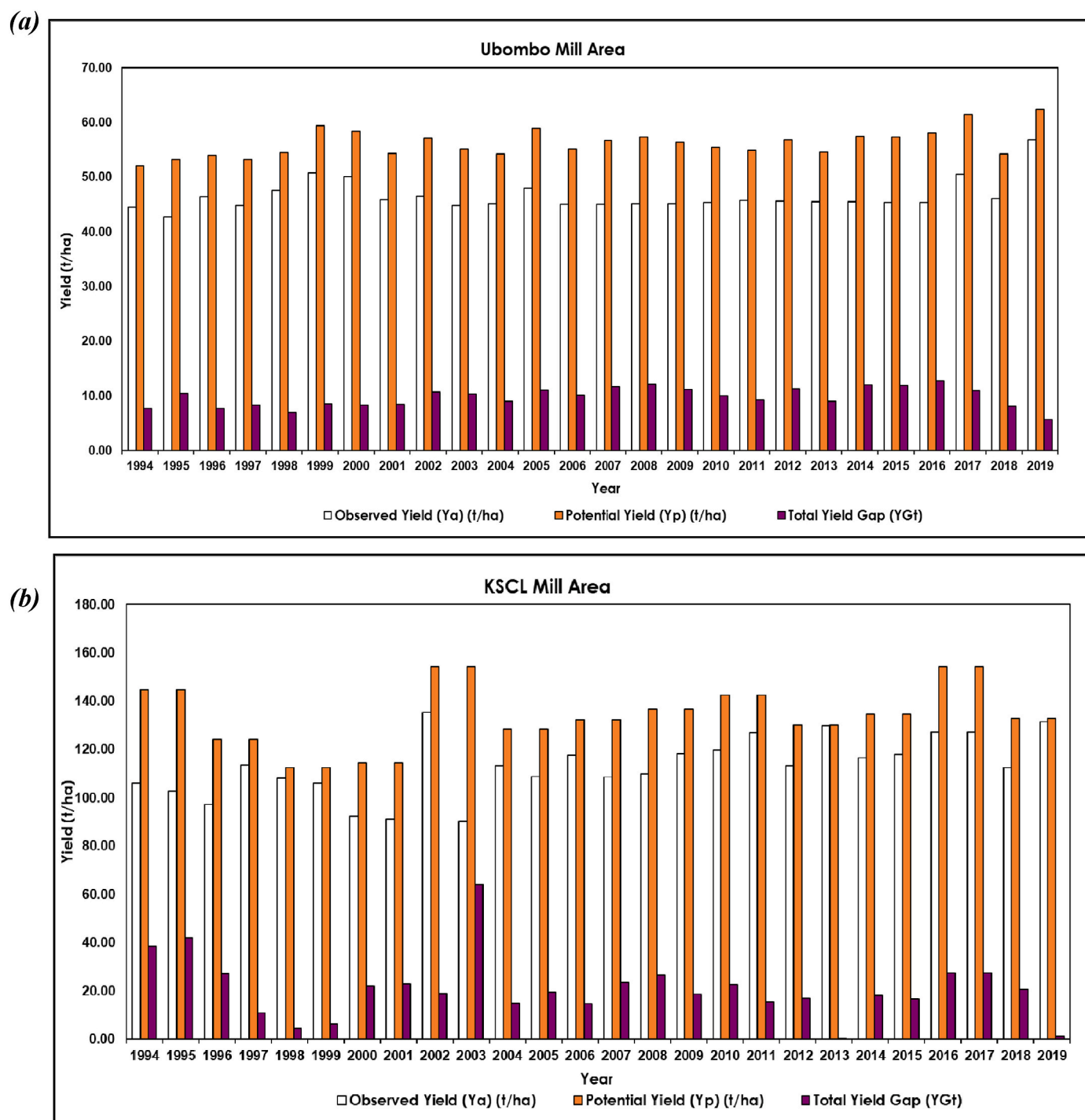
Fig. 7. (a) Observed ( Y_a ) and simulated ( Y_p ) yield for the irrigated Big Bend mill in the Ubombo catchment and (b) the KSCL mill area in the Kilombero catchment. The total yield gaps ( Y_{Gt} ) per year are also reported here indicating, on average, an increase in yield gaps over the 1996–2015 period and a subsequent decrease in yield gaps from 2016 to 2019.
