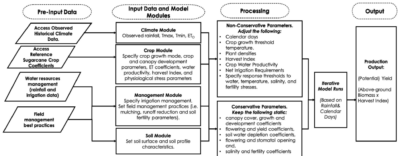
Fig. 4. A summary of the modelling procedures in the AquaCrop model adopted in this study to determine yield gaps.
