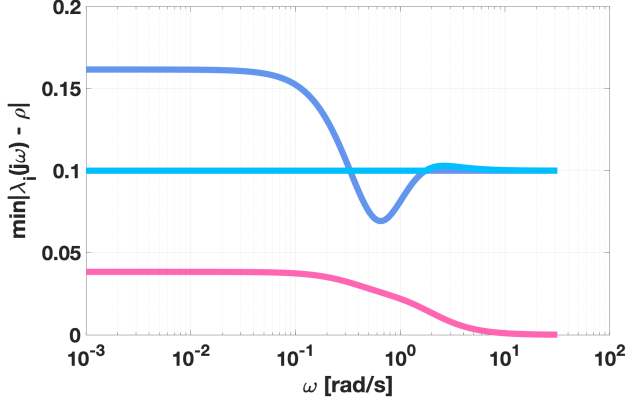
Figure 3.1: Visualisations of the stability conditions (3.7) in Theorem 5 and (3.9) in Theorem 6, for the systems in Example 1. The two blue lines are \min_{p \leq -(2\mathfrak{D})-1} |\lambda_i(j\omega) - \rho| for i = 1, 2 , with \mathfrak{D} = 5 . Nominal topology-independent stability requires that they are strictly above zero, while robust topology-independent stability requires that they are strictly above the bound \mathcal{K}(V(j\omega))\Delta_H^{max}(j\omega) shown in magenta.
