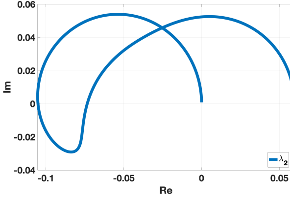
Figure 3.7: Nyquist plot of the non-zero eigenvalue \lambda_2(j\omega - \alpha) of H(j\omega - \alpha) . Since it is far from the point -1/(2\mathfrak{D}) = -1/6 , condition (3.19) is satisfied.
