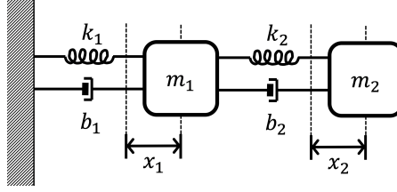
Figure 3.5: Simplified dynamic system at the nodes. The cable mass is m_1 and the road mass is m_2 ; k_i denote spring coefficients and b_i denote damping coefficients. The system is modelled as a double oscillator.
