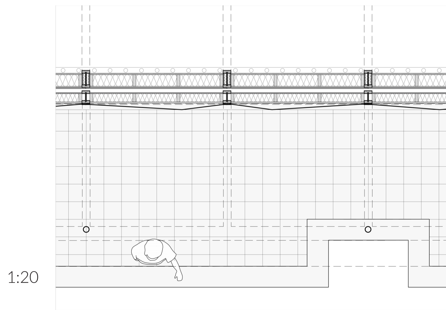
HORIZONTAL SECTION
