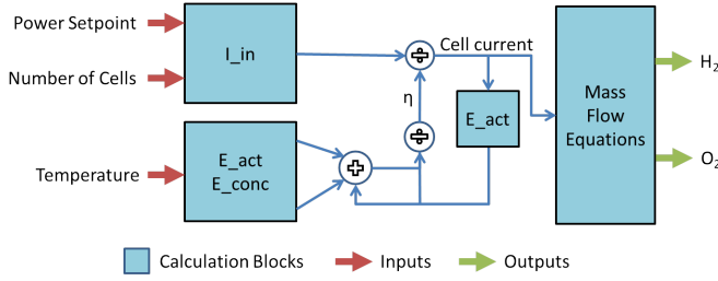
Fig. 1: electrolyzer Model
