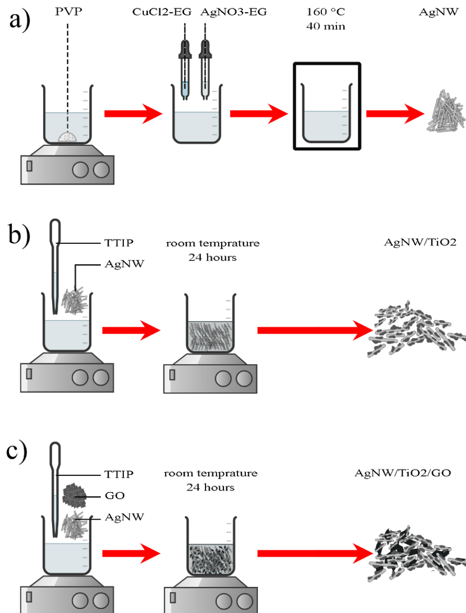
Figure 1. A schematic diagram describing the synthesis process of (a) AgNW, (b) AgNW/ \text{TiO}_2 , and (c) AgNW/ \text{TiO}_2 /GO samples.
