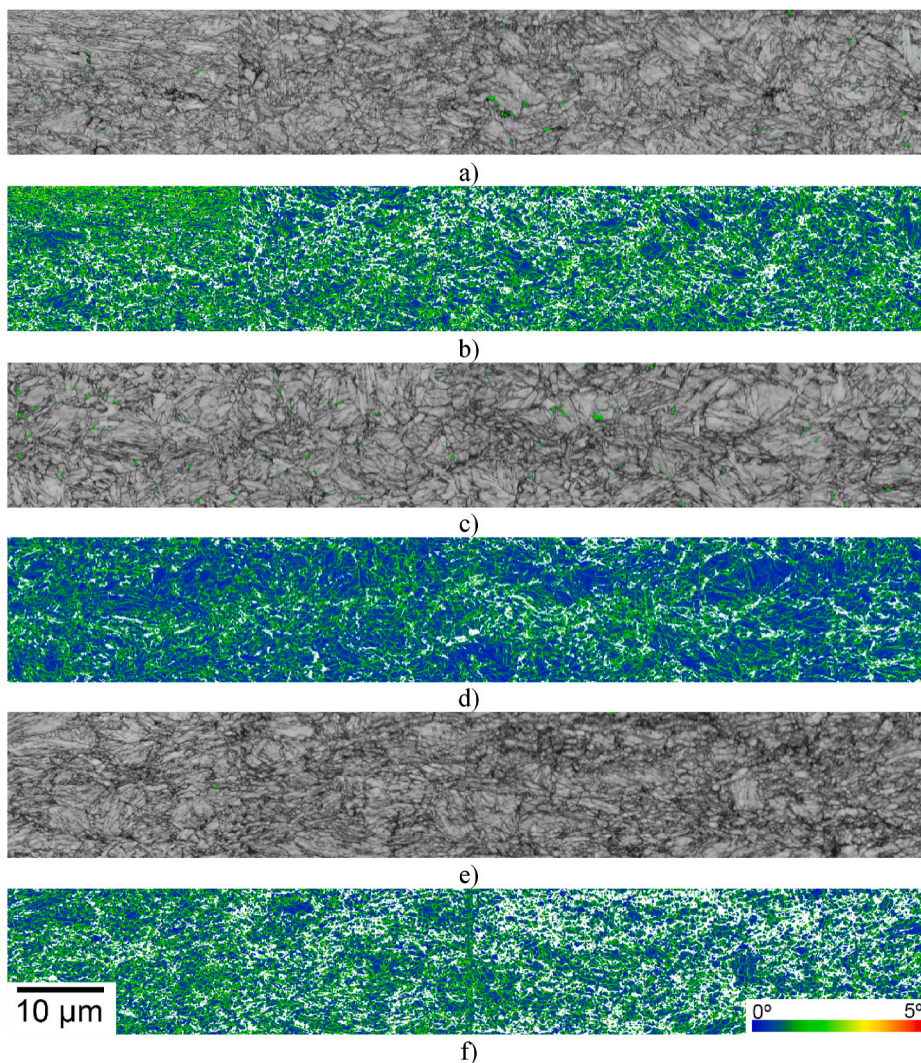
Fig. 11. Band contrast maps with overlaid phase map for base + Cr + Nb steel samples after Nakajima testing: (a, b) A010 sample, (c, d) A050 sample, (e, f) A100 sample. The scale bar 10 μm shown in (f) is valid for all maps.
