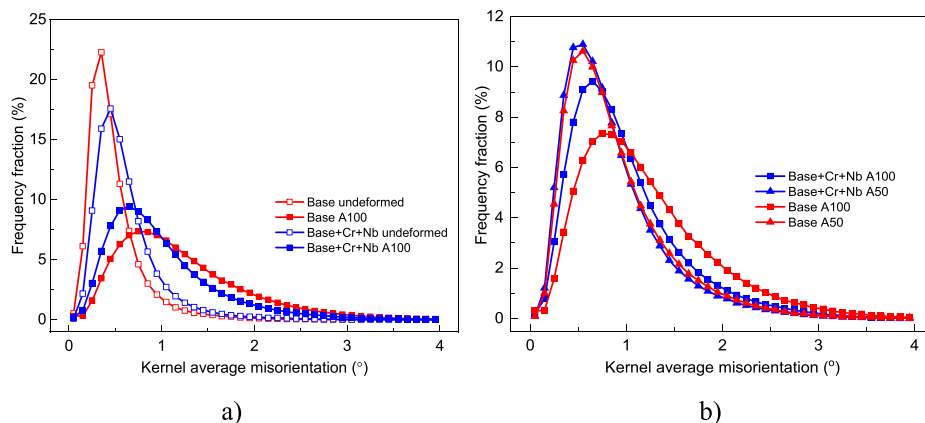
Fig. 12. a) The effect of Nakajima testing on the KAM distribution in selected samples (base and base + Cr + Nb); b) The effect of sample geometry (i.e. amount of accumulated plastic strain) on histograms of KAM distribution in selected samples (base and base + Cr + Nb).
