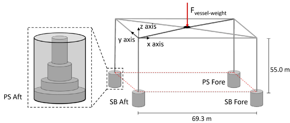
Fig. 9. Simplified structural model of the jack-up.
