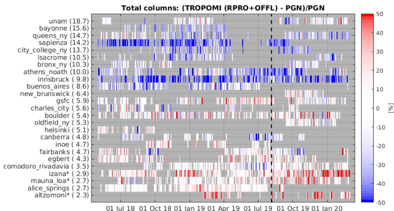
Figure 13. Percent relative difference between the S5P TROPOMI and PGN NO 2 total column data as a function of time. Stations are ordered by median NO 2 total column (lowest median value at the bottom). The dashed vertical line on 6 August 2019 represents the reduction in S5P ground pixel size from 7.0 \times 3.5 to 5.5 \times 3.5 km. The three mountaintop sites more suited for the validation of only the stratospheric column are marked with an asterisk.
