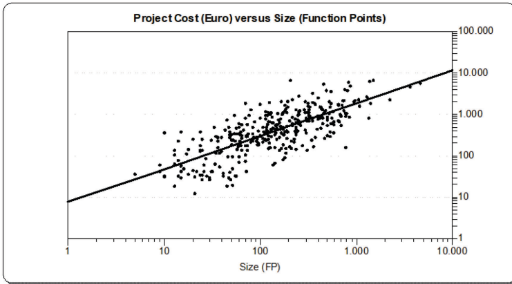
Figure 3.1: Two plotter charts representing Size (FP) versus Duration (Months) and Size (FP) versus Project Cost (Euros).
