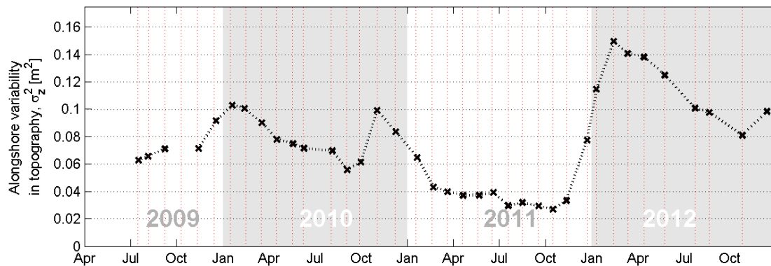
Figure 5. Bulk alongshore variability \sigma_z^2 for the 3.5 years after completion of the nourishment. Red lines indicate the survey dates. Survey of Oct. 2009 contained a data gap between the sub-aerial and sub-aqueous surveys and was therefore not used in the analysis.
