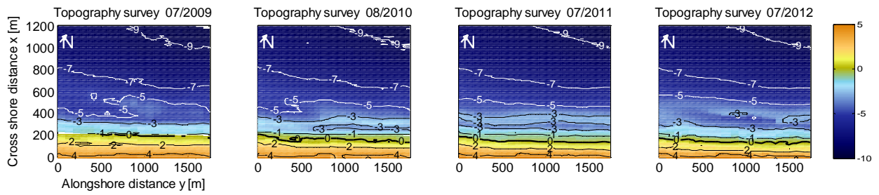
Figure 2. Vlugtenburg beach topographies in the summers of 2009 to 2012, Colors indicate bed level in meters NAP (Dutch datum at approx. MSL)
