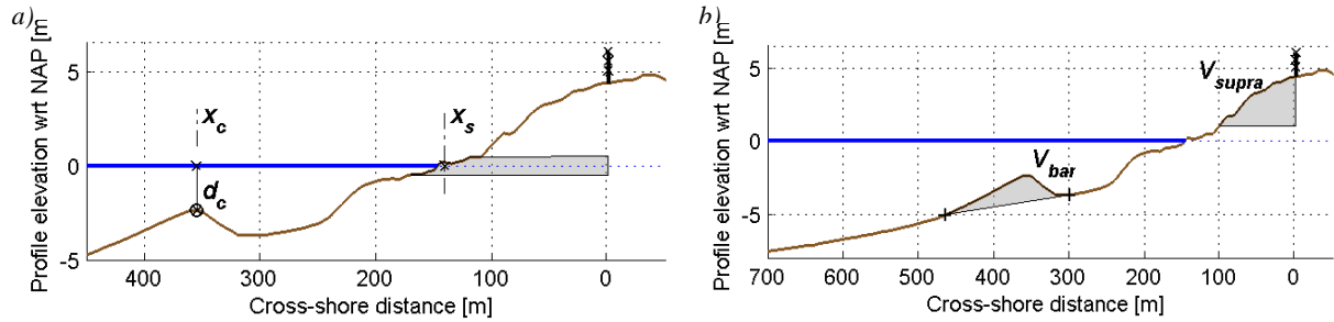
Figure 6. Profile parameters. a) Methodology to determine shoreline position x_s , bar crest location x_c and bar crest depth d_c , and b) Methodology to determine the volume of the supra tidal beach V_{supra} and the volume of the subtidal bar V_{bar} .
