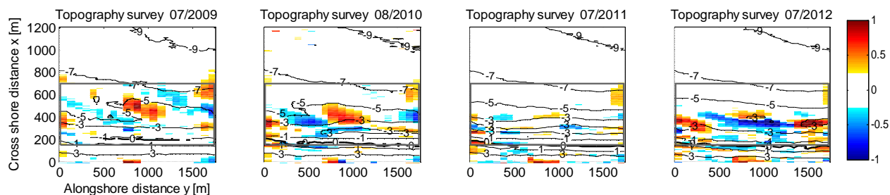
Figure 4. Planform images of alongshore variability z_{\text{var}} at Vlugtenburg beach in the summers of 2009 to 2012. Colors indicate the deviation z_{\text{var}} from the mean alongshore topography in meters. Contour levels indicate the bed level in m as displayed in Figure 2.
