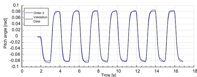
(b) Pitch angle response
