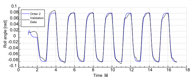
(a) Roll angle response
