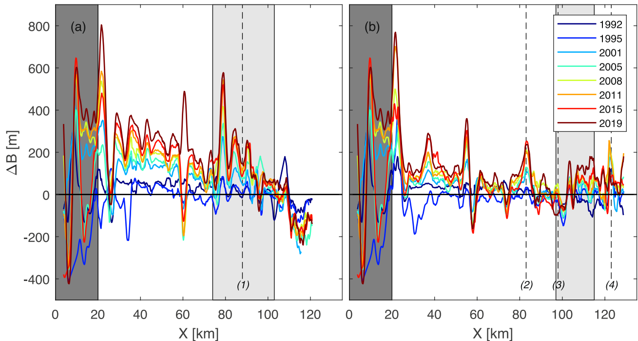
Fig. 6. Change in channel width \Delta B (in m, relative to the channel width in 1988) in the Sibsa (a) and Passur (b) rivers, derived from the satellite images in Fig. 5c. Light grey shading indicates the channel section drained by connecting channels, dark grey shading the joint Passur-Sibsa channel. The numbers refer to the location of gauging stations, where 1 = S88, 2 = P83 (Mongla), 3 = P98, and 4 = P123 (Khulna).
