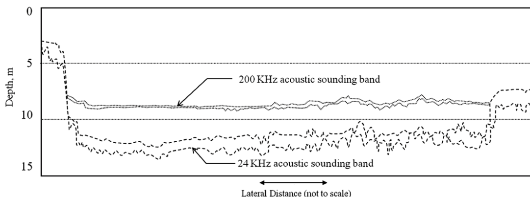
Figure 2: Dual-frequency echo sounding in a channel with fluid mud layers. From Alexander et al. (1997)
