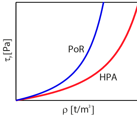
Figure 9: Non-linear relationship between the yield stress \tau_y and the density \rho of mud
