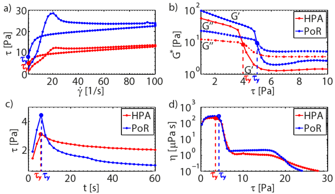
Figure 8: Rheological methods for determining the yield stress \tau_y of fluid mud at the Port of Rotterdam and the Hamburg Port Authority. a) Thixotropy of mud measured by controlled shear rate experiment. b) Amplitude sweep experiment. c) Stress grow experiment. d) Controlled stress sweep experiment.
