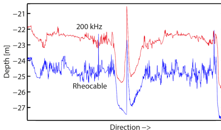
Figure 6: Correlation of the high frequency echo sounding (200 kHz) and Rheocable measurements after water injection dredging in the Port of Rotterdam.
