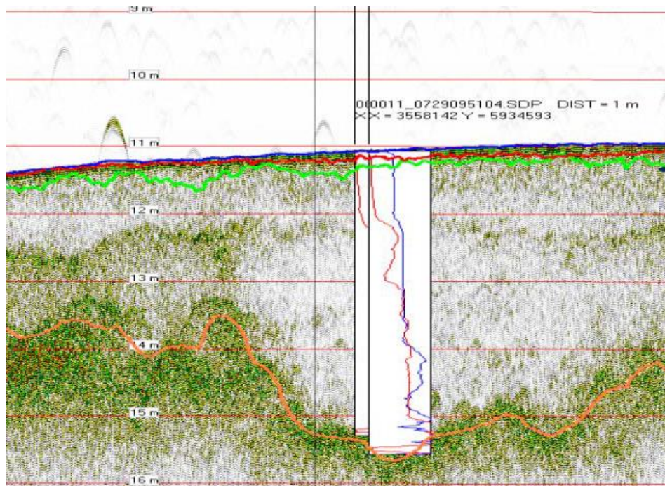
Figure 4: The Rheotune 'calibration' to the measured acoustics signal using SILAS in Hamburg.
