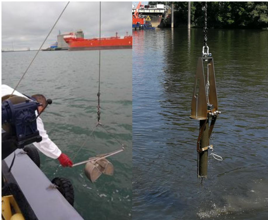
Figure 7: Disturbed (left) and undisturbed (right) sampling methods
