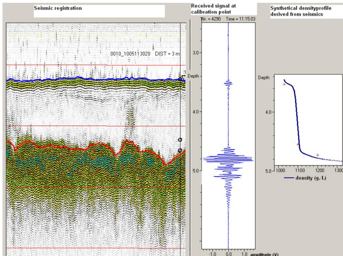
Figure 3: The density 'calibration' to the measured acoustic signal using SILAS From Diaferia et al. (2013)
