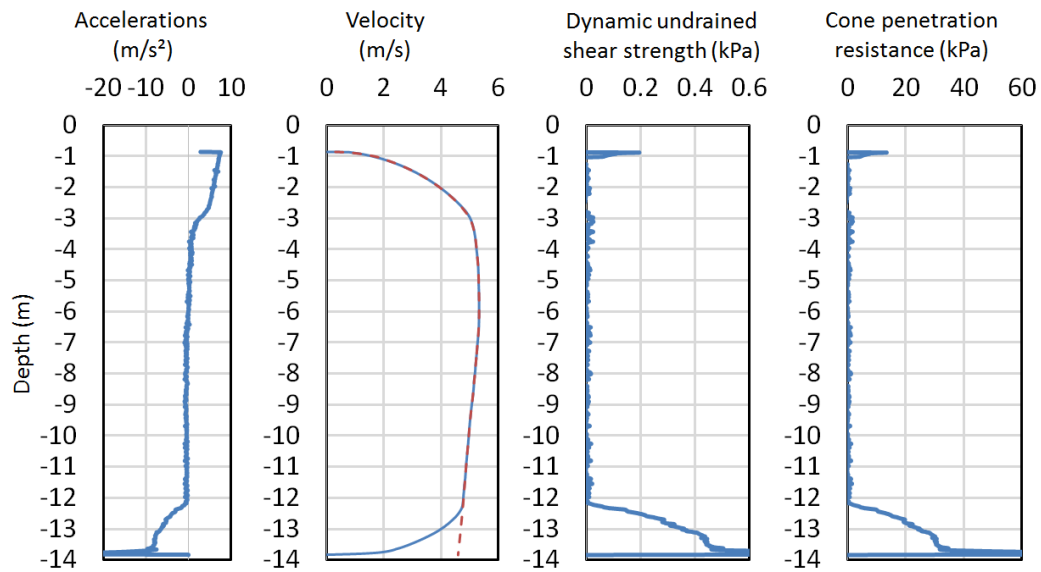
Figure 5: The data measured by the Graviprobe. The fluid mud layer is detected at the depth of -12 m
