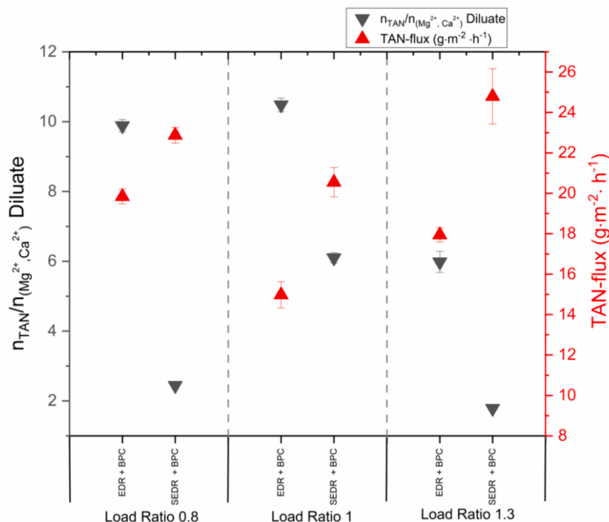
Fig. 7. On the left y-axis, the molar ratio of TAN to cations ( \text{Mg}^{2+} and \text{Ca}^{2+} ) in the diluate is represented as \eta_{\text{TAN}}/\eta_{\text{cations}} . The right y-axis displays the average TAN flux in grams per square meter per hour ( \text{g}\cdot\text{m}^{-2}\cdot\text{h}^{-1} ). The values are presented for the EDR + BPC and SEDR + BPC configurations across various load ratios indicated on the x-axis.
