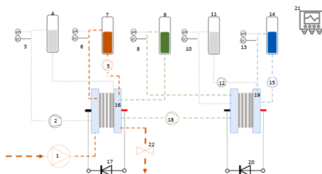
Fig. 3. The used experimental set-up comprised of an EDR/SEDR cell with feed and bleed (16), a BPC/BPMED cell (19), feeding pump (1), two power supplies (17, 20), recirculating diaphragm pumps (2, 5, 18, 12, 15), pH and EC sensors (3, 6, 8, 10, 13), recirculation vessels (4, 7, 9, 11, 14), a data logger (21) and a “bleed” phase draining valve (22).
