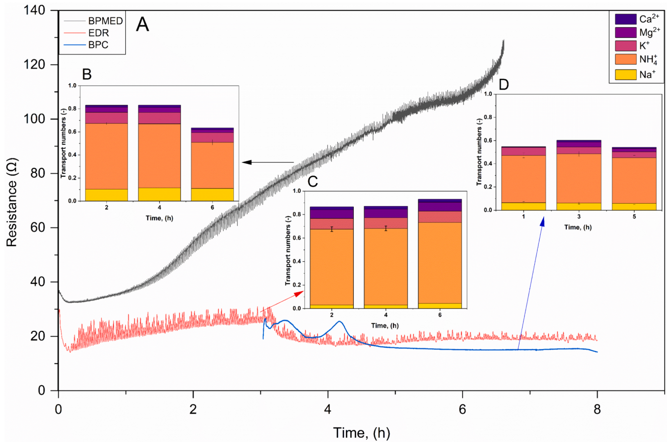
Fig. 4. A: Progression of electrical resistance (Ω) of the stacks measured as voltage-to-current ratio (V/I) for the BPMED and EDR + BPC configurations at an applied L_N of 1. The y-axis represents the resistance (values expressed in ohm (Ω)) for both configurations, while the x-axis denotes the operation time in hours. B: The transport numbers of cations in BPMED indicated with a black arrow. C: The transport numbers of cations in EDR indicated with a red arrow. D: The transport numbers of cations in BPC indicated with a blue arrow.
