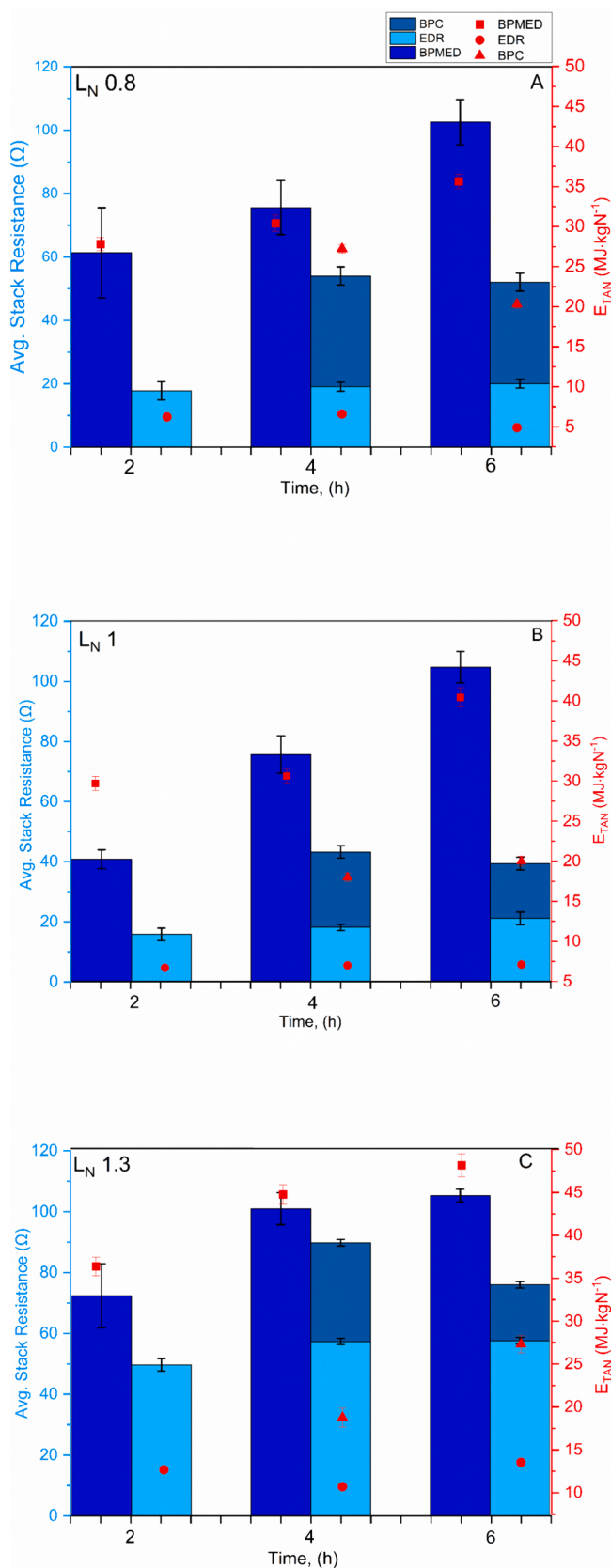
Fig. 5. The resistance and energy consumption of BPMED and EDR + BPC for all the applied load ratios. The average resistance of the stacks is indicated on the left y-axis with shades of blue colour by the stacked columns. On the right y-axis is indicated the energy consumption with shapes of red colour by the scatter diagram. Graph A: L_N = 0.8 , B: L_N = 1 and C: L_N = 1.3 .
