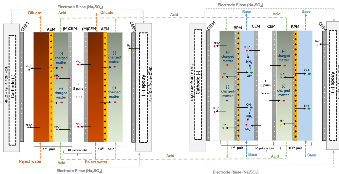
Fig. 2. Schematic representation of the used combination of ED and BPC. Left unit represents the ED concept, which involves a pair of membranes consisting of an AEM and a CEM for EDR. When the stack was operated as SEDR, the CEM was replaced with an MSCEM. The reject water is introduced into the diluate chamber, and as the process progresses, cations such as TAN and negatively charged matter are transported into the acid chamber. The acid chamber becomes at the same time the concentrate for the EDR and the feed for BPC. Within the base chamber, the concentrated TAN reacts with \text{OH}^- generated by the BPM, resulting in the formation of \text{NH}_3 .
