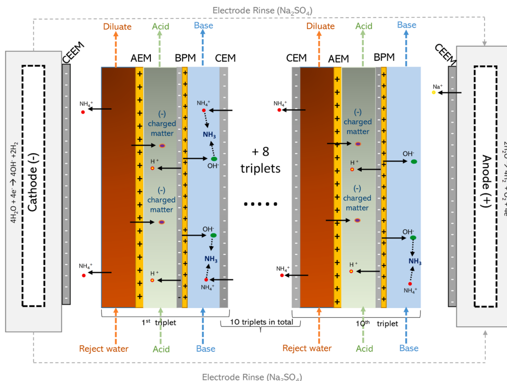
Fig. 1. Schematic representation of the membrane configuration in the used conventional BPMED stack. The reject water is introduced into the diluate chamber, and the applied current initiates the transport of cations, including TAN, towards the base chamber while anions, represented by negatively charged organic matter, are transported to the acid chamber. Simultaneously, the BPM facilitates the water splitting, resulting in the generation of H^+ and OH^- ions. Due to their respective charges, the H^+ ions are directed towards the acid compartment, contributing to the formation of an acidic solution, while the OH^- ions migrate towards the base chamber, leading to the formation of a base solution.
