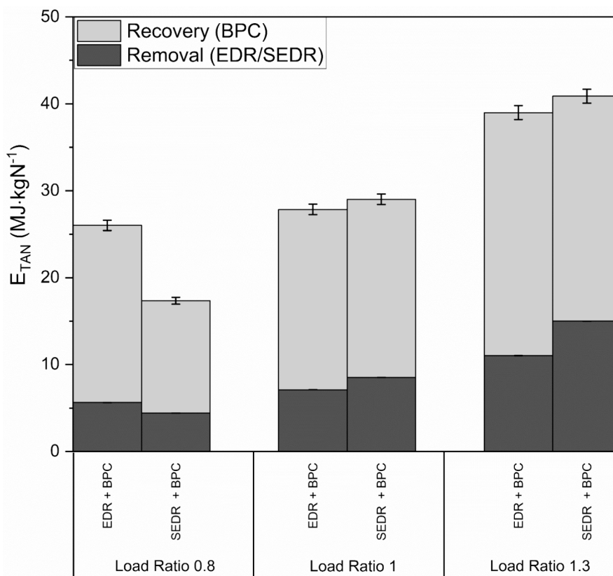
Fig. 9. E_{TAN} in MJ·kgN -1 for removal and recovery by EDR + BPC and SEDR + BPC at an L_N of 0.8, 1 and, 1.3.
