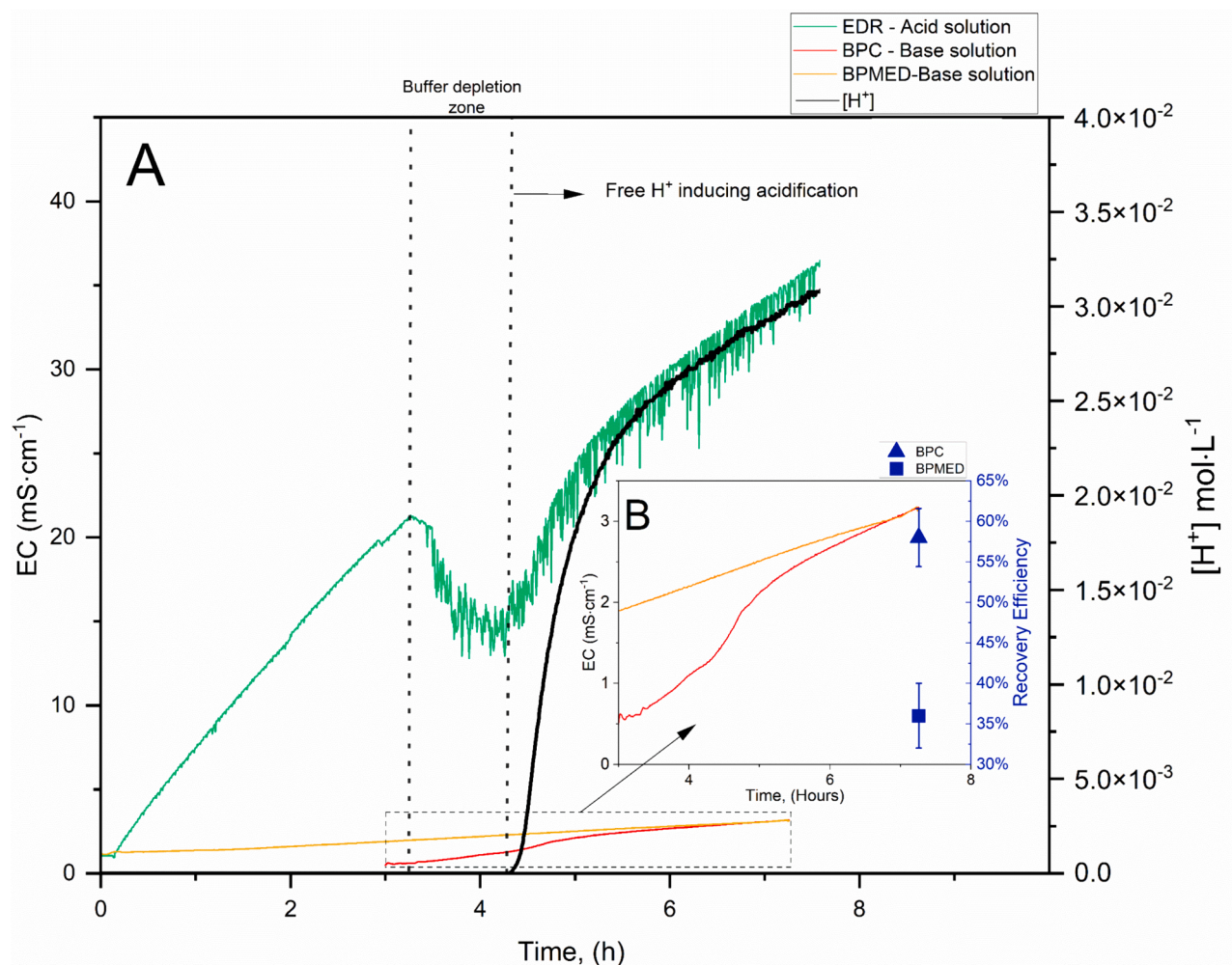
Fig. 6. The concentration gradient expressed as electrical conductivity and the recovery efficiency for EDR + BPC and BPMED, applying an L_N of 1. A: EC in \text{mS}\cdot\text{cm}^{-1} for acid and base. The left y-axis indicates the EC of the acid concentrate solution and the right y-axis depicts the free \text{H}^+ as molarity. The x-axis corresponds to the time in hours. The produced \text{CO}_2 caused the oscillations on the EC sensors which is observed after the activation of the BPC at 3 h once the target of 20\text{ mS}\cdot\text{cm}^{-1} be the EDR in the acid was reached. B: The left y-axis indicates the EC in \text{mS}\cdot\text{cm}^{-1} and the right y-axis the recovery efficiency in (%) for BPMED and BPC in the base solution. The error bars of the recovery efficiency values correspond to minimum and maximum values.
