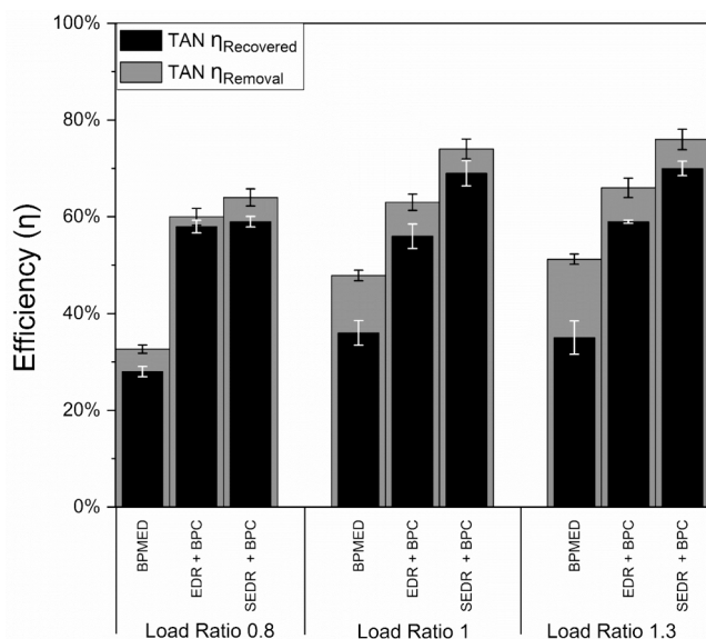
Fig. 8. The \eta of TAN in % from reject water achieved by BP MED, EDR + BPC and, SEDR + BPC at L_N 0.8, 1 and 1.3.
