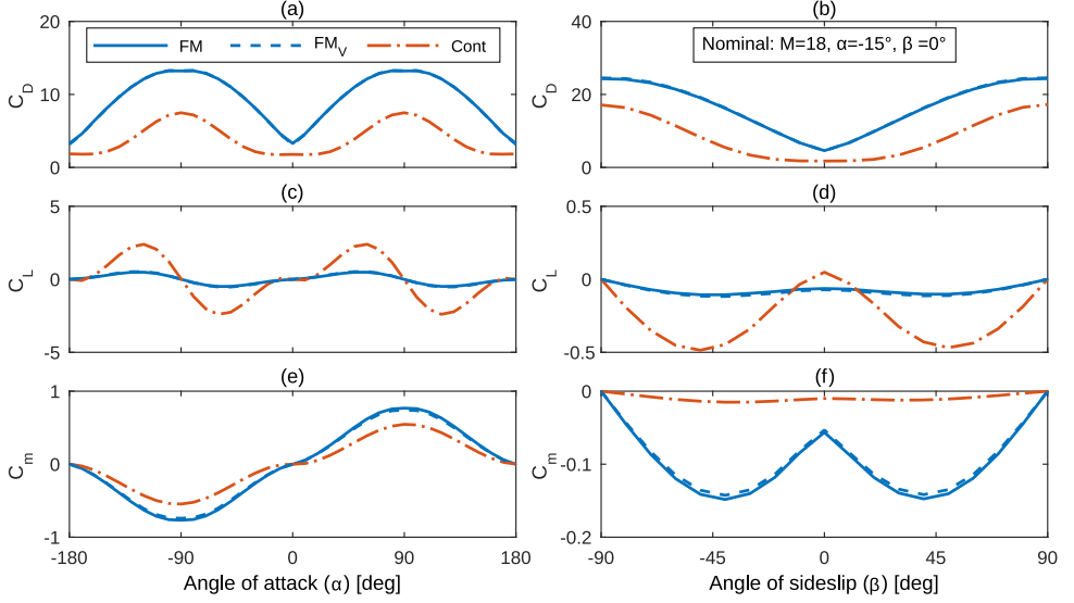
Figure 4.2: Selection of aerodynamic force and moment coefficients for GOCE for the free-molecular (FM) regime and continuum (Cont) regime, including an externally produced source FM_V for verification.
