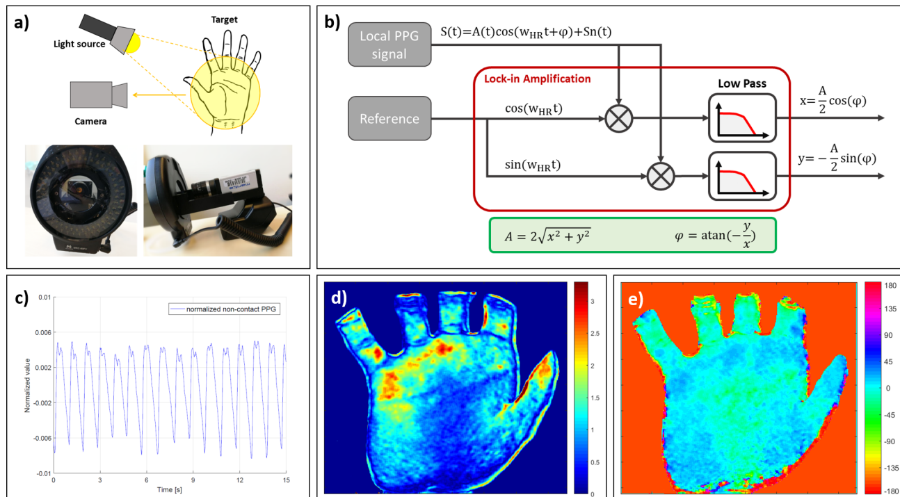
Figure 1. a) Setup for PPG imaging acquisition, composed of a camera and a light source. b) Block diagram of the Lock-In amplification algorithm for extracting the perfusion map. c) Normalized PPG signal from the entire region of interest. d) PPG Amplitude map. e) PPG phase map.
