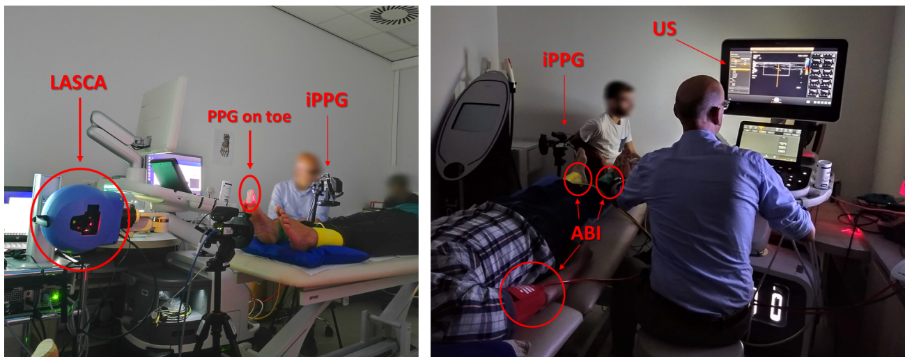
Figure 4. Setup of the experiments. The volunteer lies on the bed, cuffs are positioned around their arm and legs. All the used measurements devices are displaced around and indicated.
